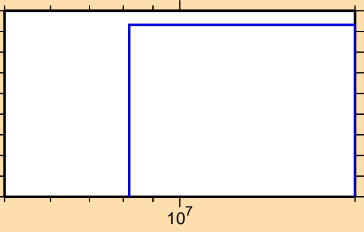
\sigma vs. E for ^{137}\text{Pm}(n,2n\alpha)
