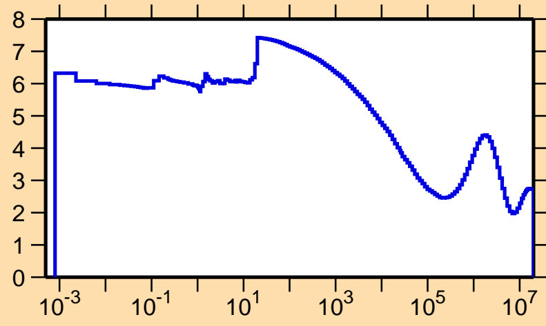
\sigma vs. E for ^{138}\text{Pm}(n,\text{el.})
