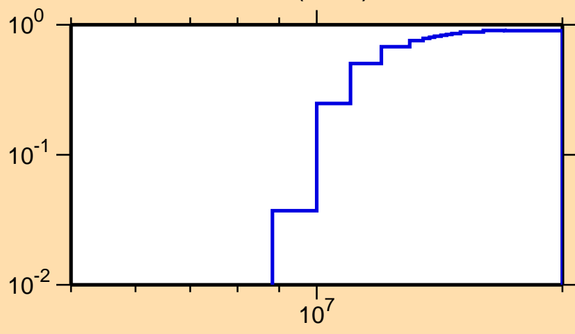
\sigma vs. E for ^{138}\text{Pm}(n,2n)
