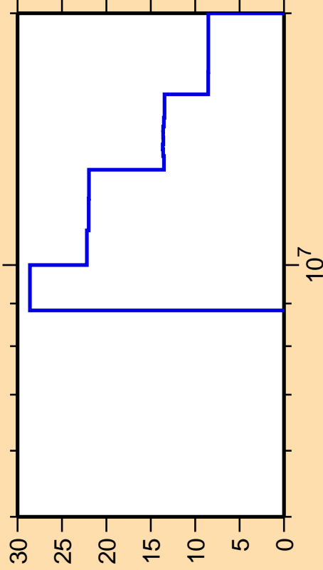
\Delta\sigma/\sigma vs. E for ^{138}\text{Pm}(n,2n)
