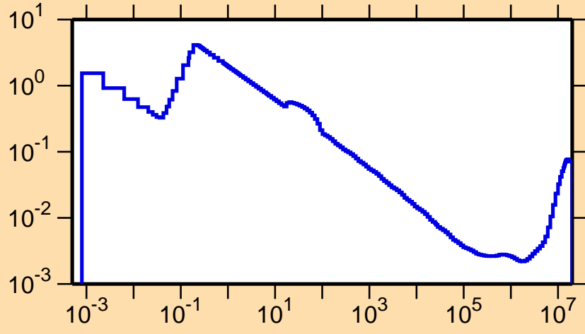
\sigma vs. E for ^{138}\text{Pm}(n,\alpha)
