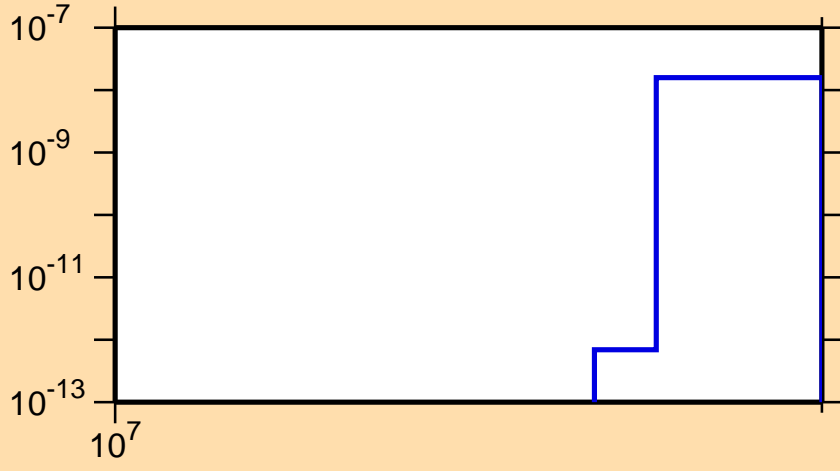
\sigma vs. E for ^{138}\text{Pm}(n,nt)
