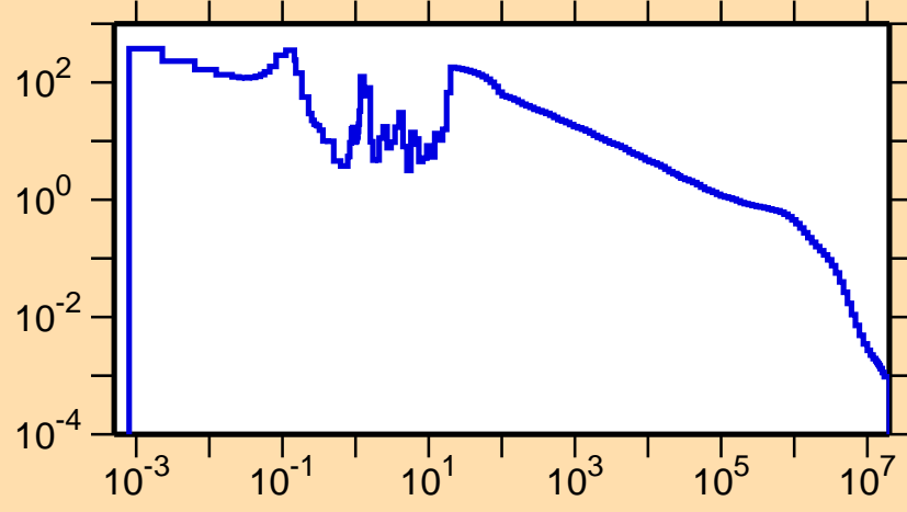
\sigma vs. E for ^{138}\text{Pm}(n,\gamma)
