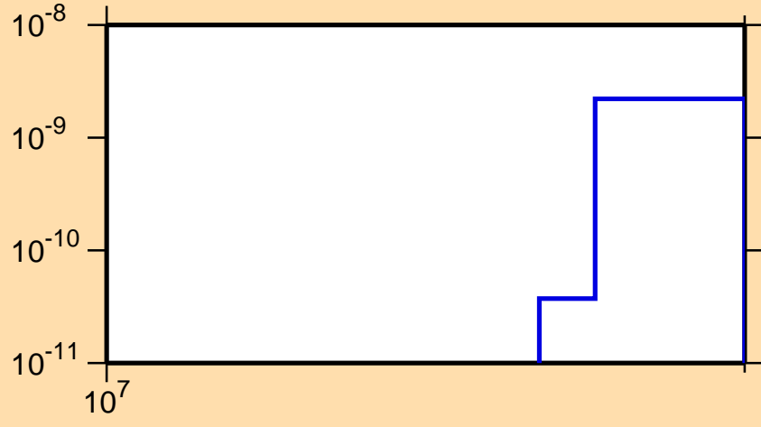
\sigma vs. E for ^{138}\text{Pm} (mt 34)
