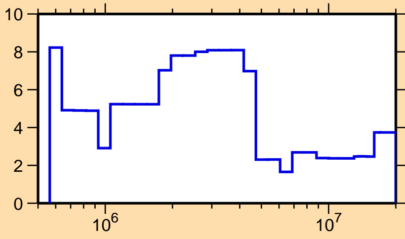
\Delta\sigma/\sigma vs. E for ^{138}\text{Pm}(n,\text{el.})
