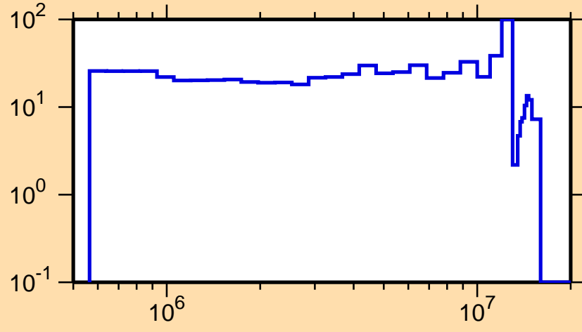
\Delta\sigma/\sigma vs. E for ^{138}\text{Pm}(n,n_1)
