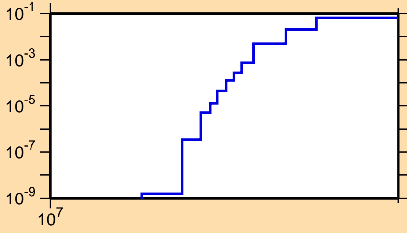
\sigma vs. E for ^{138}\text{Pm}(n,2np)
