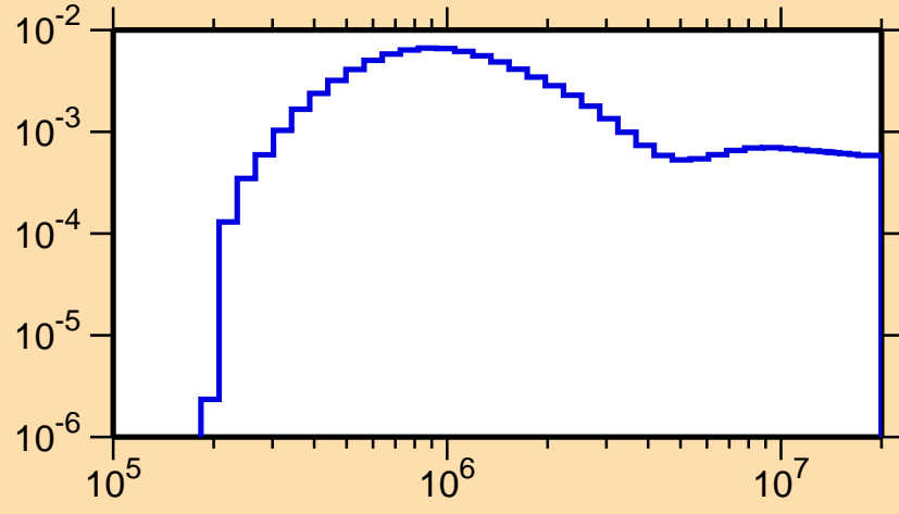
\sigma vs. E for ^{138}\text{Pm}(n,n_3)
