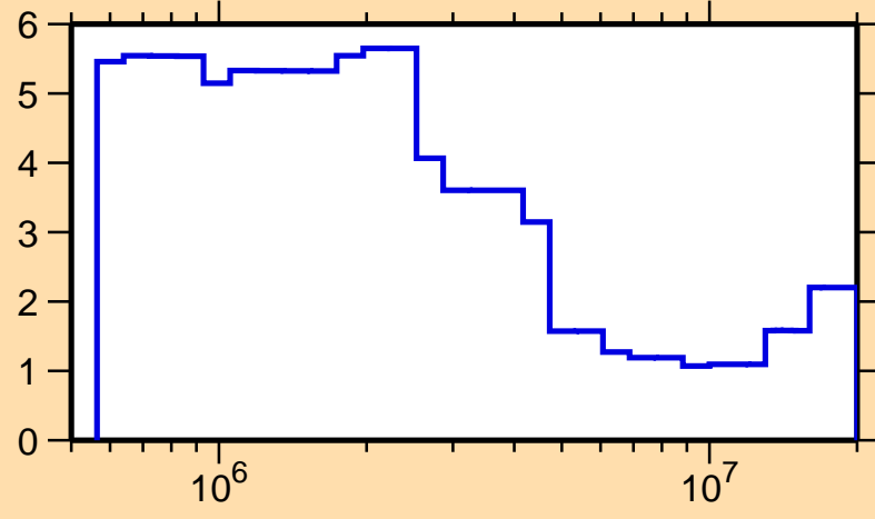
\Delta\sigma/\sigma vs. E for ^{138}\text{Pm}(n,\text{tot.})
