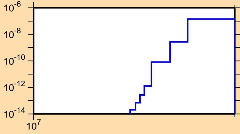
\sigma vs. E for ^{138}\text{Pm}(n,pt)
