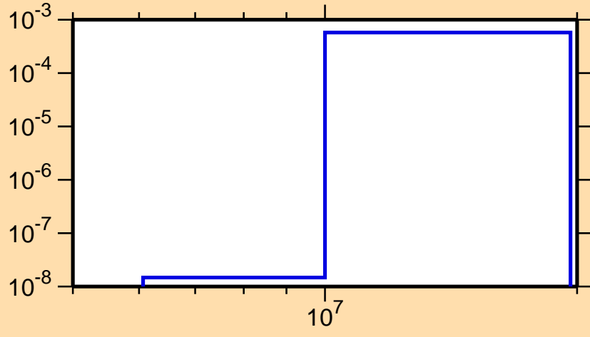
\sigma vs. E for ^{138}\text{Pm}(n,t)
