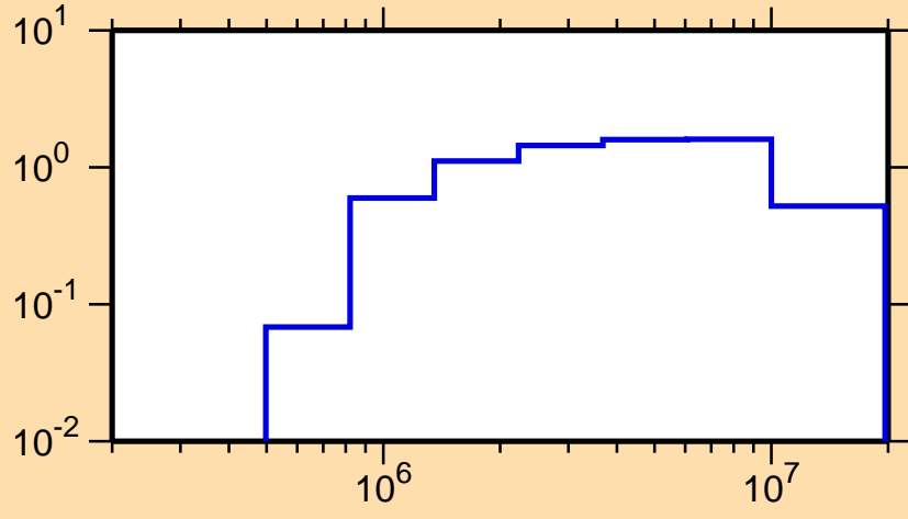
\sigma vs. E for ^{138}\text{Pm}(n,n\text{cont.})
