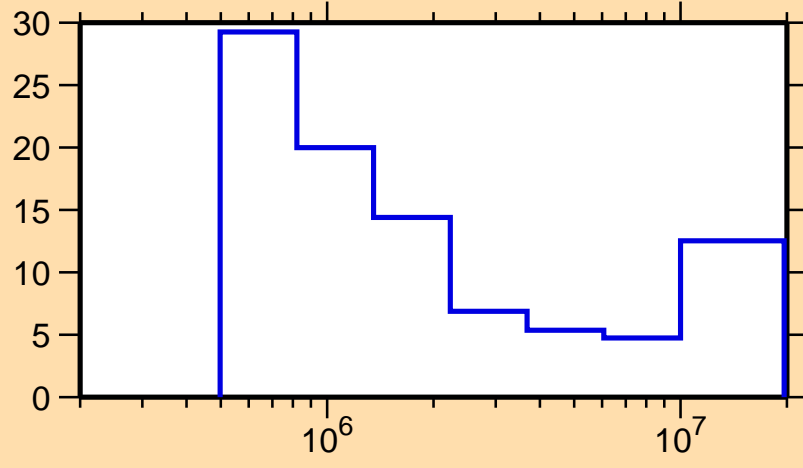
\Delta\sigma/\sigma vs. E for ^{138}\text{Pm}(n,n\text{cont.})
