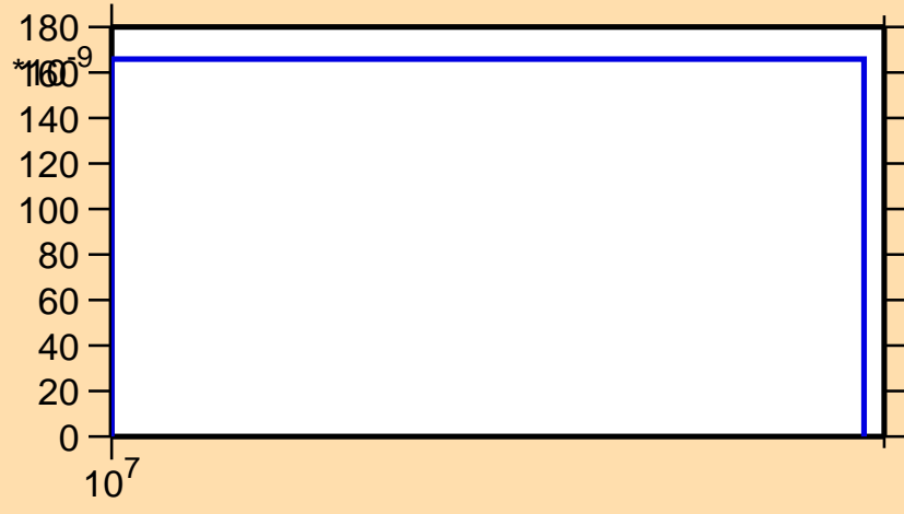
\sigma vs. E for ^{138}\text{Pm}(n,2n\alpha)
