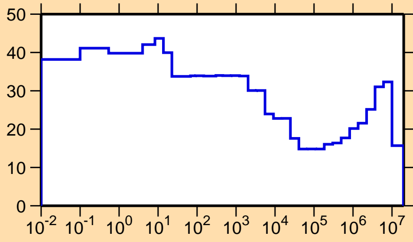
\Delta\sigma/\sigma vs. E for ^{138}\text{Pm}(n,p)
