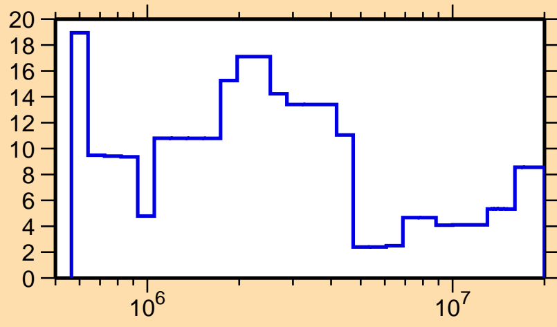
\Delta\sigma/\sigma vs. E for ^{138}\text{Pm}(n,\text{tot.})
