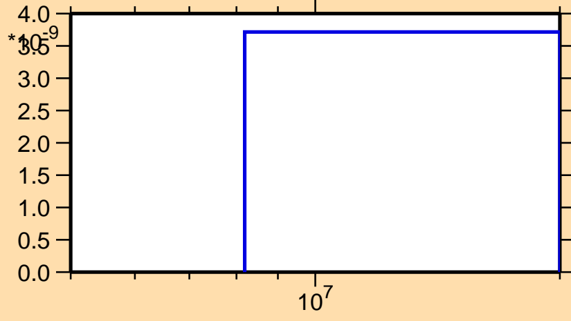
\sigma vs. E for ^{138}\text{Pm}(n,\text{pt})
