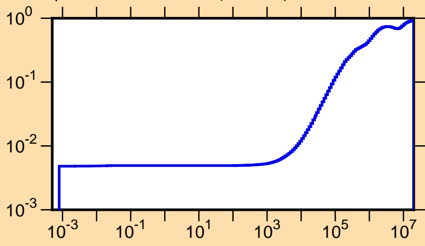
\mu vs. E for ^{140}\text{Pm}(\text{mt251})
