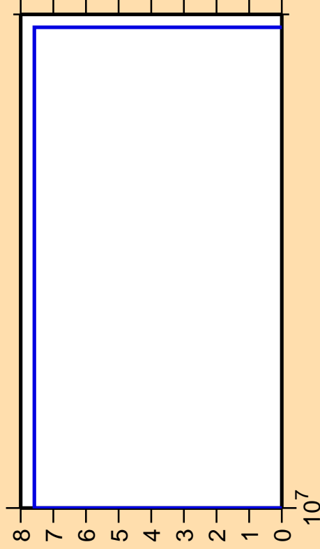
\Delta\sigma/\sigma vs. E for ^{140}\text{Pm}(\text{mt117})
