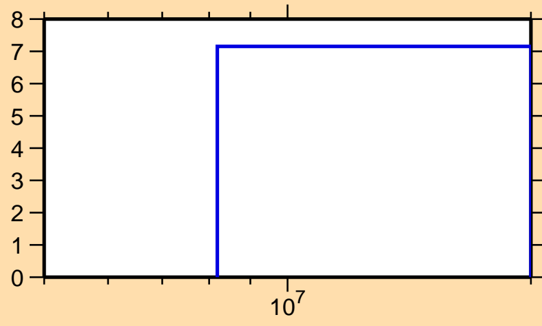
\Delta\sigma/\sigma vs. E for ^{140}\text{Pm}(n,el.)
