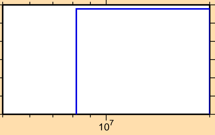
\sigma vs. E for ^{140}\text{Pm}(n,2n\alpha)
