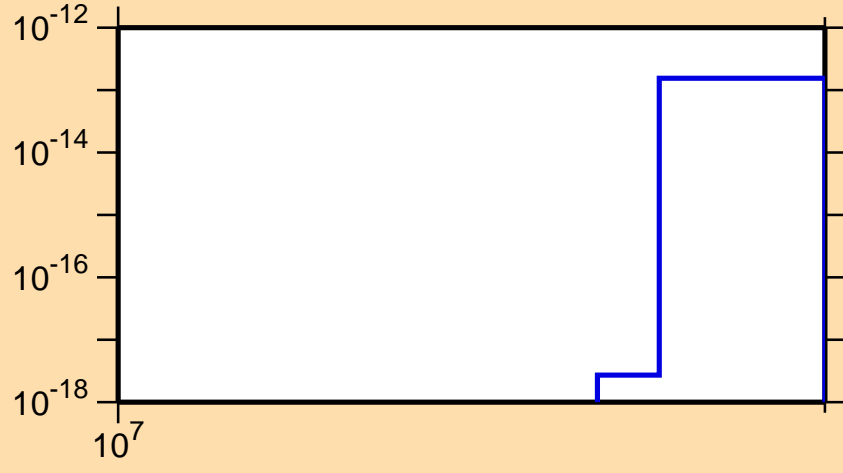
\sigma vs. E for ^{141}\text{Pm}(n,pt)
