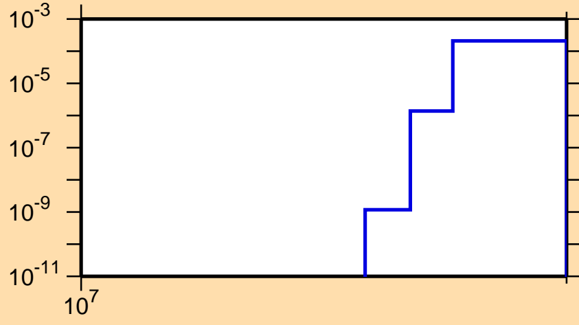
\sigma vs. E for ^{141}\text{Pm}(n,2np)
