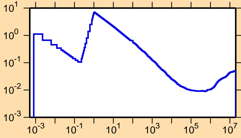
\sigma vs. E for ^{141}\text{Pm}(n,p)
