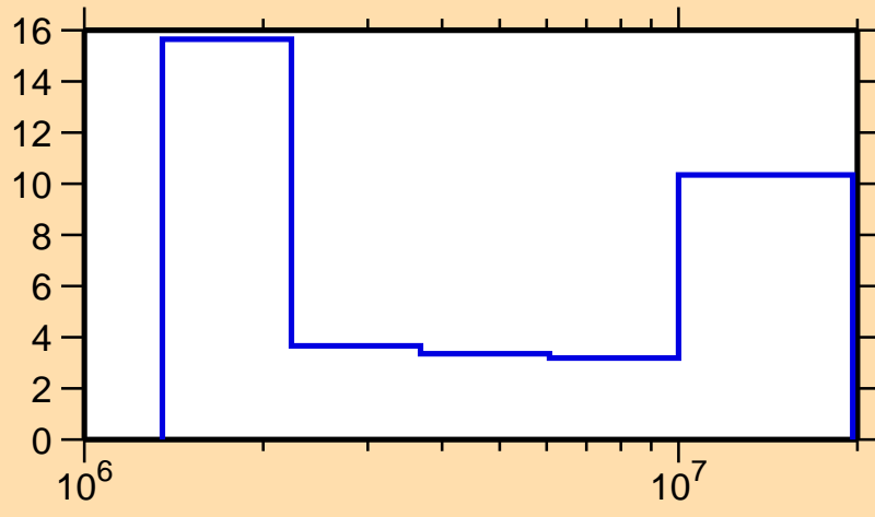
\Delta\sigma/\sigma vs. E for ^{141}\text{Pm}(n,ncont.)
