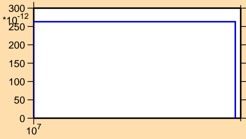
\sigma vs. E for ^{141}\text{Pm}(n,\text{pd})
