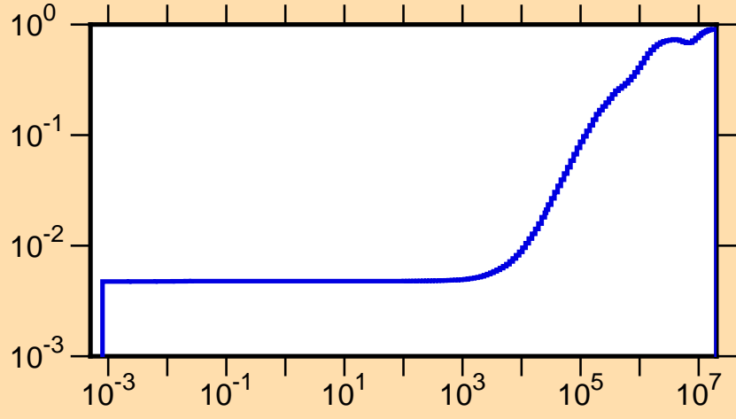
\mu vs. E for ^{142}\text{Pm}(\text{mt251})
