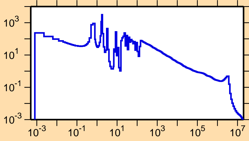
\sigma vs. E for ^{142}\text{Pm}(n,\gamma)
