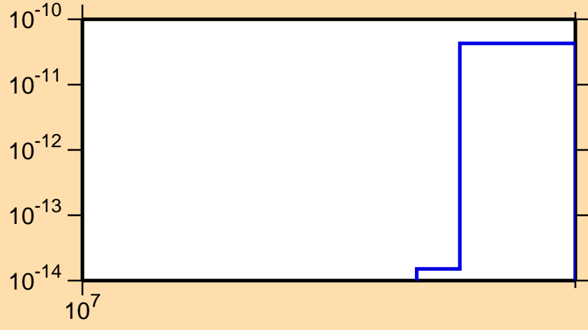
\sigma vs. E for ^{142}\text{Pm}(n,pt)
