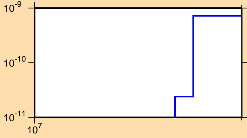
\sigma vs. E for ^{142}\text{Pm}(n,\text{pd})
