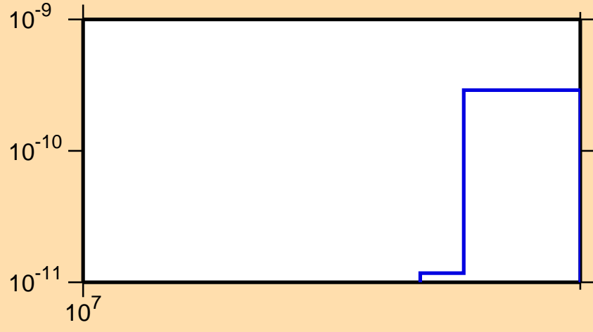
\sigma vs. E for ^{142}\text{Pm} (mt 45)
