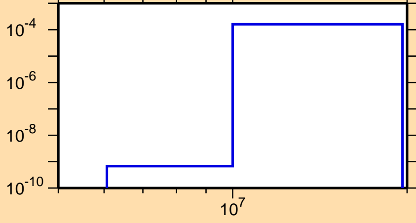
\sigma vs. E for ^{142}\text{Pm}(n,t)
