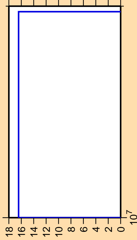
\Delta\sigma/\sigma vs. E for ^{142}\text{Pm}(n,pd)
