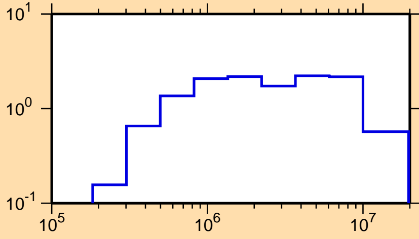
\sigma vs. E for ^{142}\text{Pm}(n,\text{inel.})
