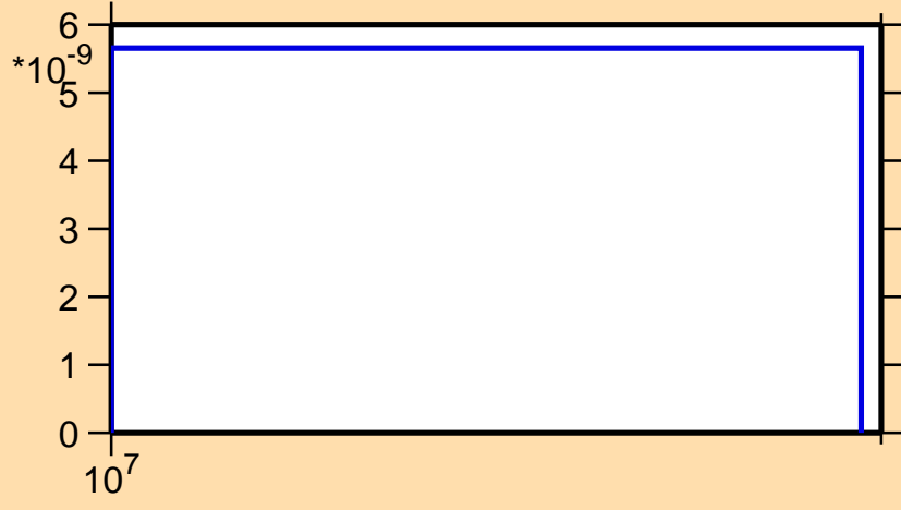
\sigma vs. E for ^{142}\text{Pm}(n,2n\alpha)
