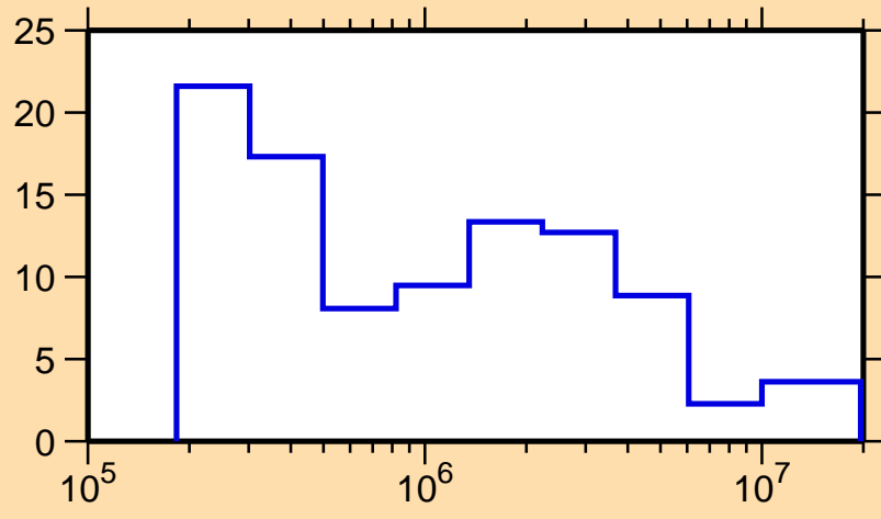
\Delta\sigma/\sigma vs. E for ^{142}\text{Pm}(n,\text{tot.})
