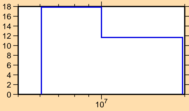
\Delta\sigma/\sigma vs. E for ^{142}\text{Pm}(n,2n)
