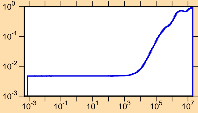
\mu vs. E for ^{143}\text{Pm}(\text{mt251})
