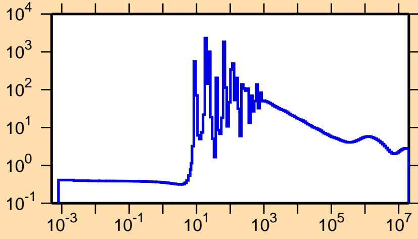
\sigma vs. E for ^{143}\text{Pm}(n,\text{el.})
