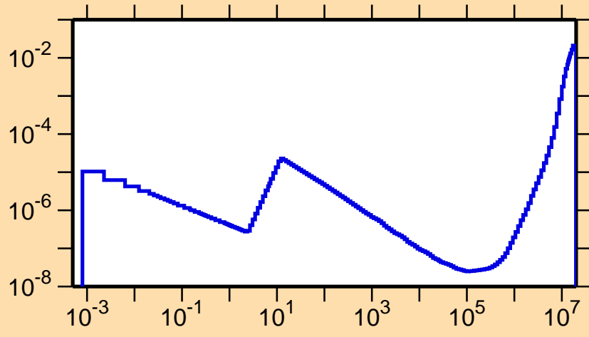
\sigma vs. E for ^{143}\text{Pm}(n,\alpha)
