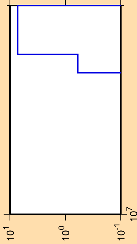
\Delta\sigma/\sigma vs. E for ^{143}\text{Pm}(\text{mt117})
