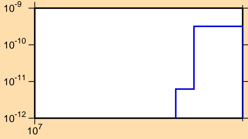
\sigma vs. E for ^{143}\text{Pm}(n,pd)
