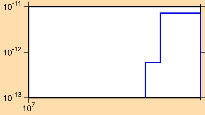
\sigma vs. E for ^{143}\text{Pm}(\text{mt117})
