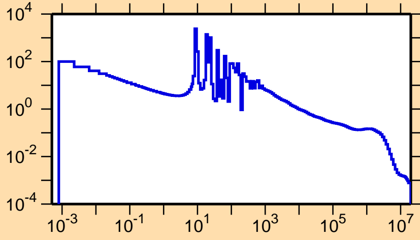
\sigma vs. E for ^{143}\text{Pm}(n,\gamma)
