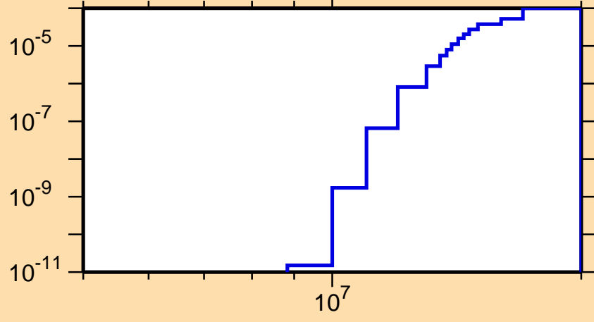
\sigma vs. E for ^{146}\text{Pm}(n,2n\alpha)
