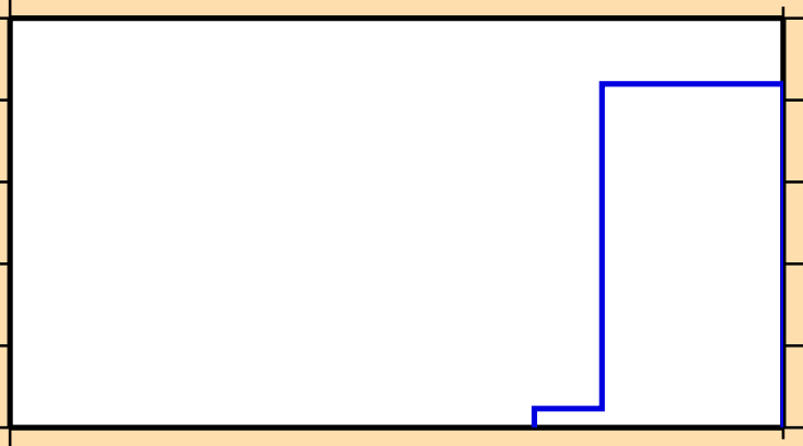
\sigma vs. E for ^{146}\text{Pm} (mt 11)
