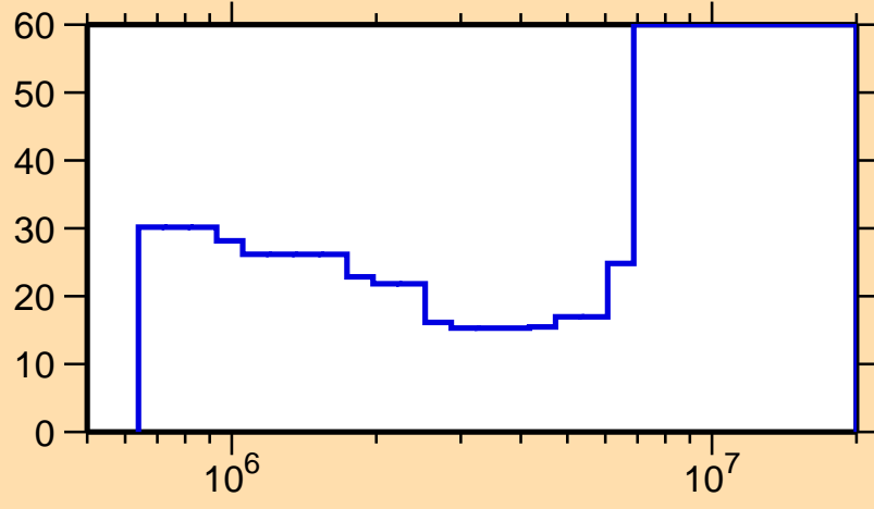
\Delta\sigma/\sigma vs. E for ^{146}\text{Pm}(n,\text{inel.})
