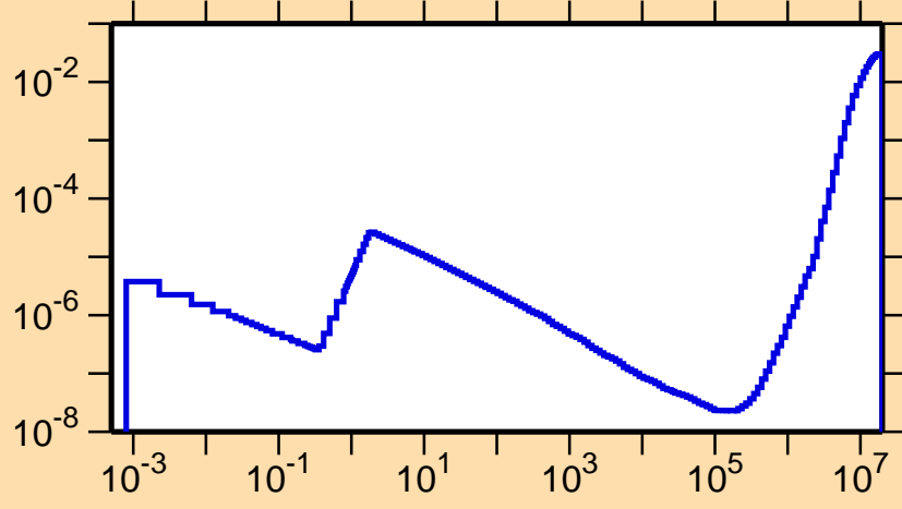
\sigma vs. E for ^{146}\text{Pm}(n,p)
