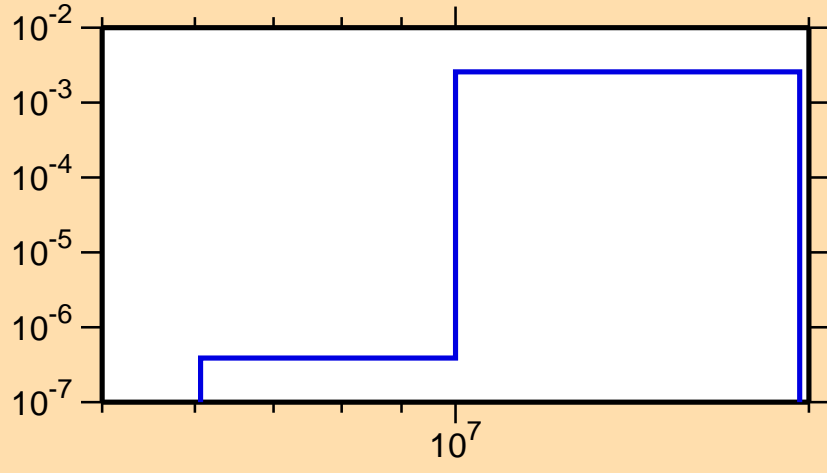
\sigma vs. E for ^{146}\text{Pm}(n,np)
