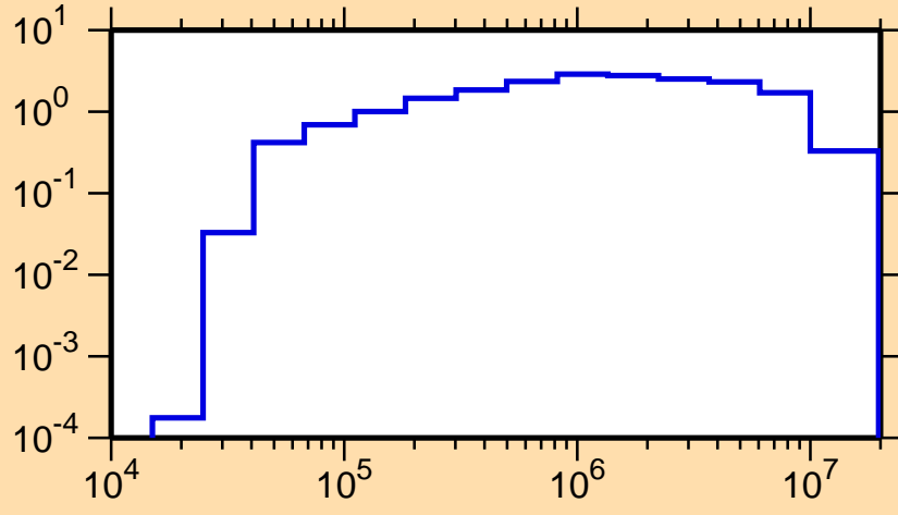
\sigma vs. E for ^{146}\text{Pm}(n,\text{inel.})
