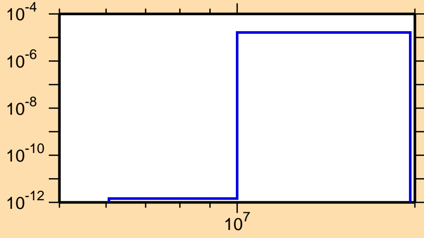
\sigma vs. E for ^{146}\text{Pm}(n,2n\alpha)
