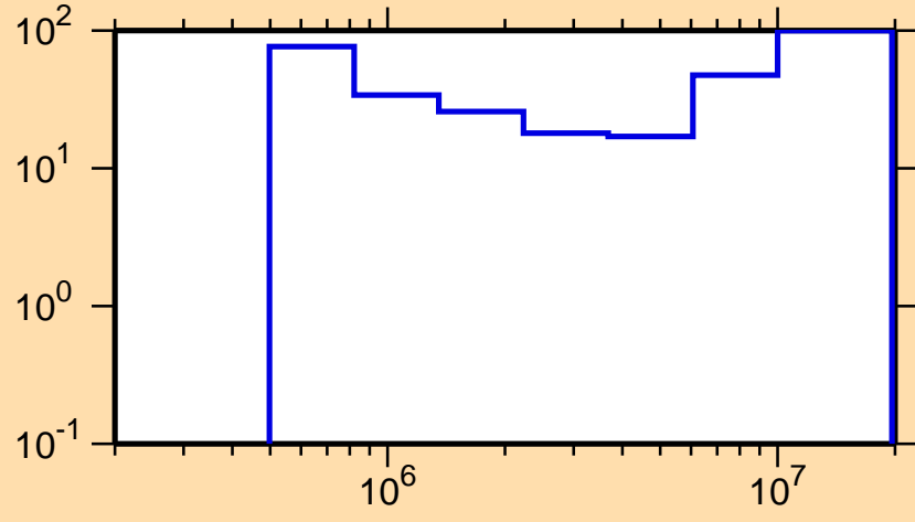
\Delta\sigma/\sigma vs. E for ^{146}\text{Pm}(n,ncont.)
