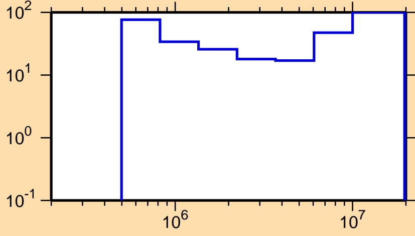
\Delta\sigma/\sigma vs. E for ^{146}\text{Pm}(n,n\text{cont.})
