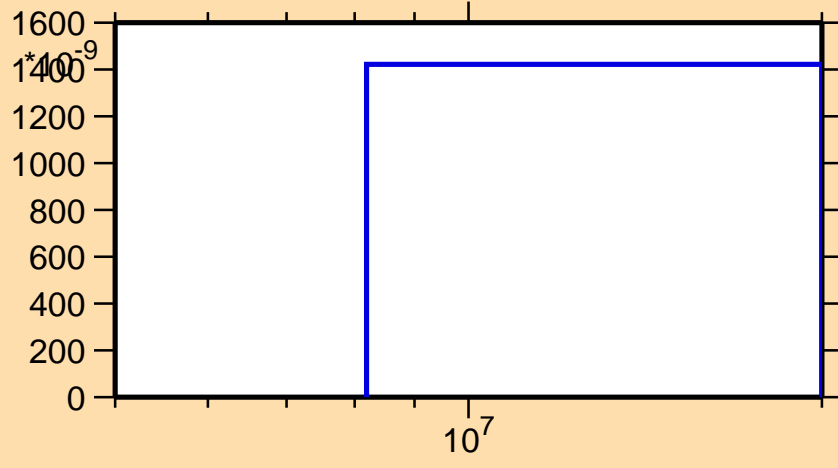
\sigma vs. E for ^{146}\text{Pm}(n,2np)
