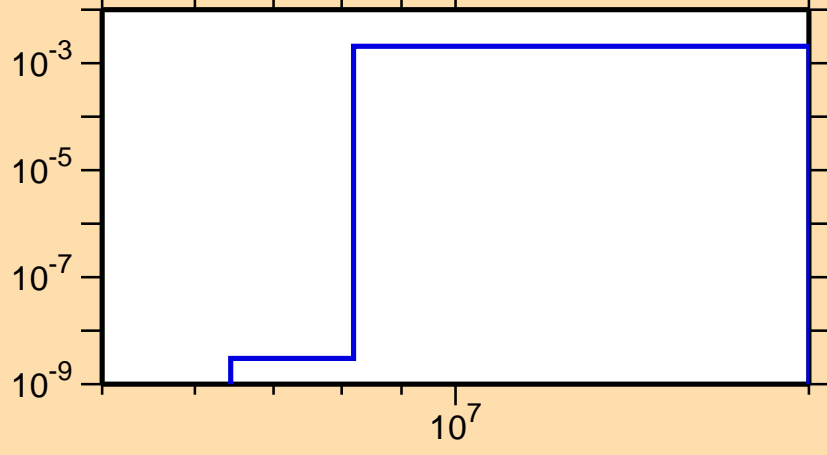
\sigma vs. E for ^{146}\text{Pm}(n,np)
