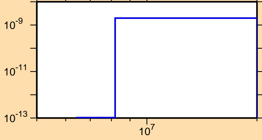
\sigma vs. E for ^{146}\text{Pm}(n,p\alpha)
