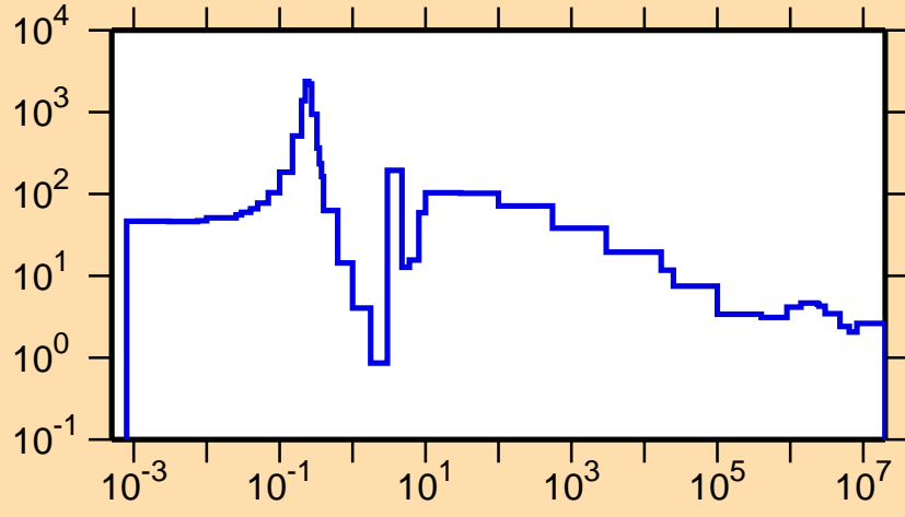
\sigma vs. E for ^{146}\text{Pm}(n,\text{el.})
