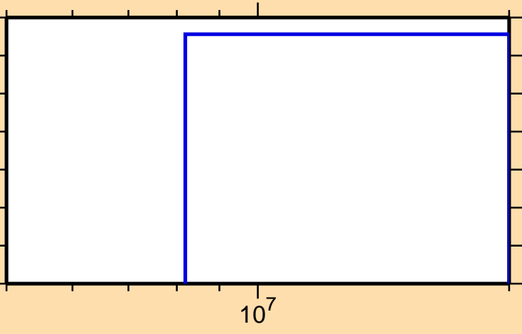
\sigma vs. E for ^{146}\text{Pm}(n,2n\alpha)
