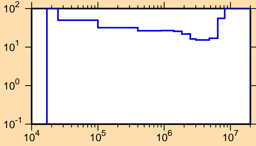
\Delta\sigma/\sigma vs. E for ^{146}\text{Pm}(n,\text{inel.})
