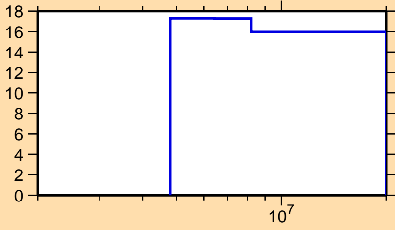
\Delta\sigma/\sigma vs. E for ^{146}\text{Pm}(n,\text{tot.})
