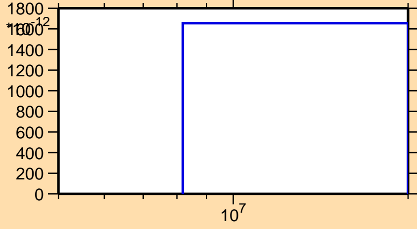
\sigma vs. E for ^{146}\text{Pm}(n,\text{He}3)
