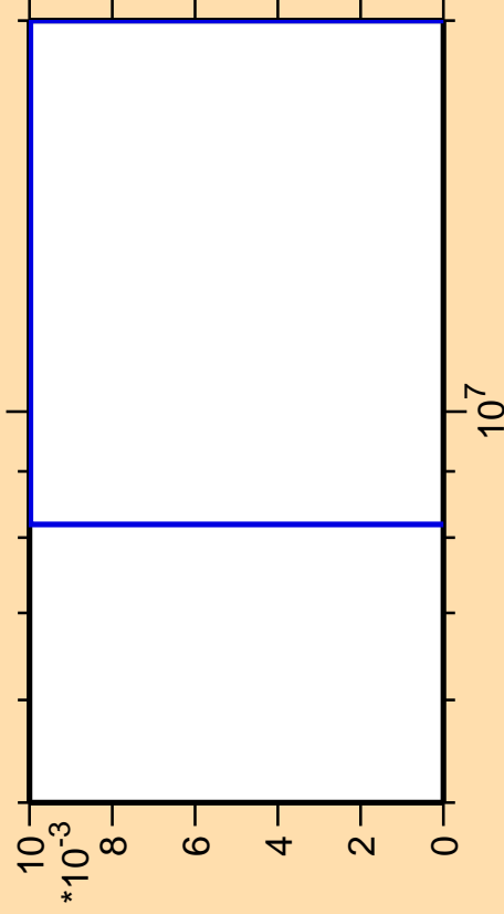
\Delta\sigma/\sigma vs. E for ^{146}\text{Pm} (mt 11)
