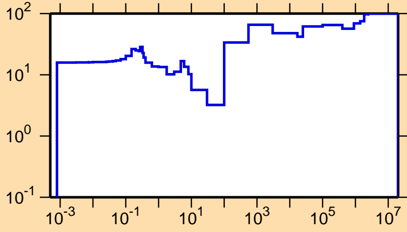
\Delta\sigma/\sigma vs. E for ^{146}\text{Pm}(n,\gamma)
