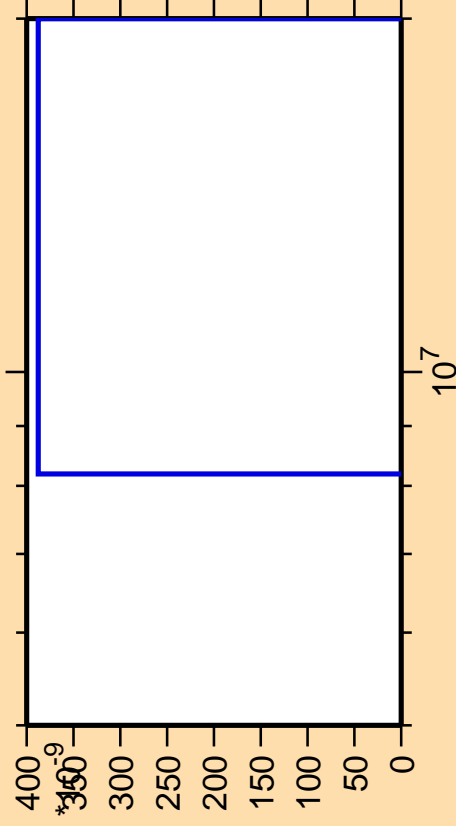
\Delta\sigma/\sigma vs. E for ^{146}\text{Pm} (mt 42)
