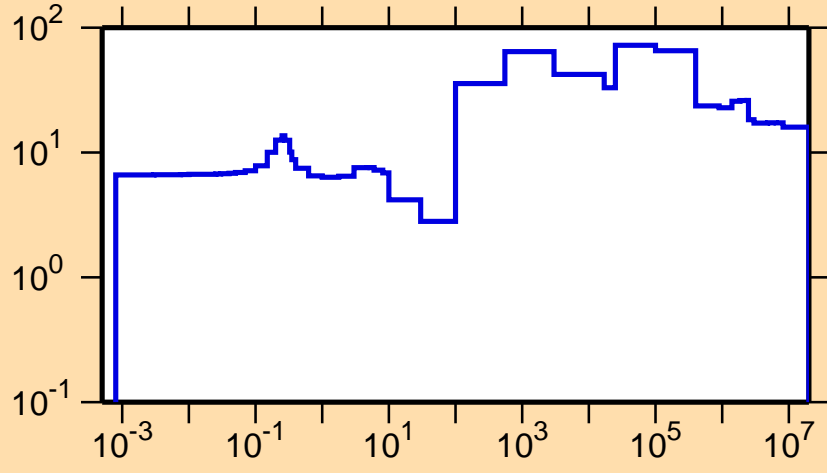
\Delta\sigma/\sigma vs. E for ^{146}\text{Pm}(n,\text{tot.})
