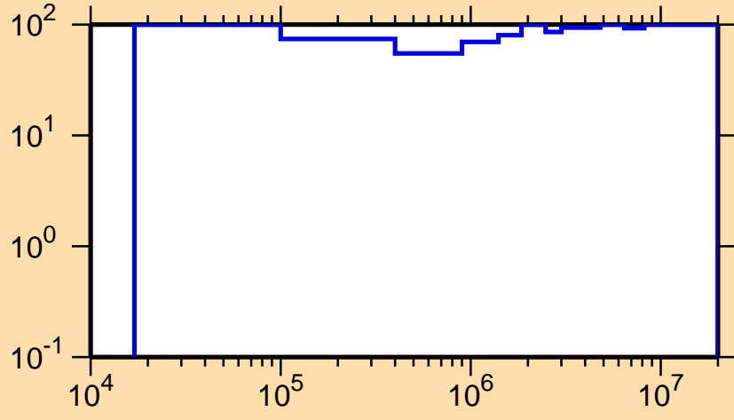
\Delta\sigma/\sigma vs. E for ^{146}\text{Pm}(n,n_1)
