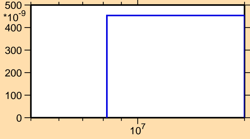
\sigma vs. E for ^{146}\text{Pm}(n,nt)
