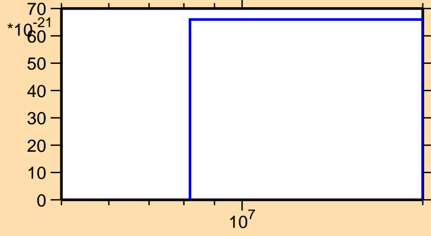
\sigma vs. E for ^{146}\text{Pm} (mt 42)
