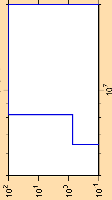
\Delta\sigma/\sigma vs. E for ^{146}\text{Pm}(n,p\alpha)
