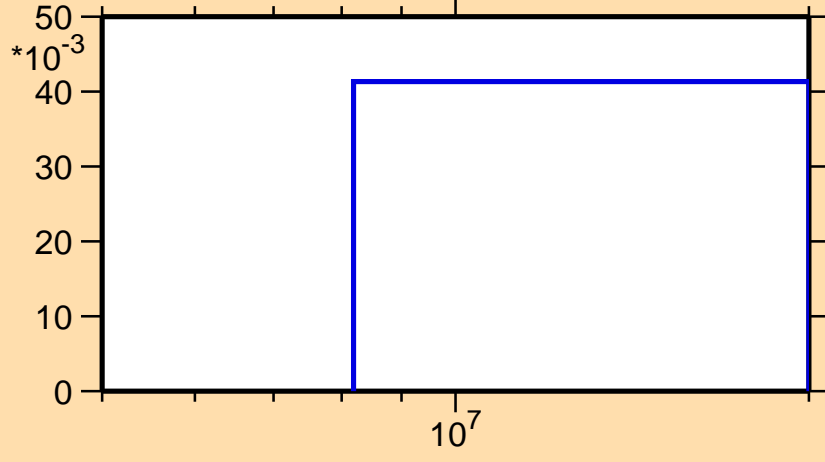
\sigma vs. E for ^{146}\text{Pm}(n,3n)
