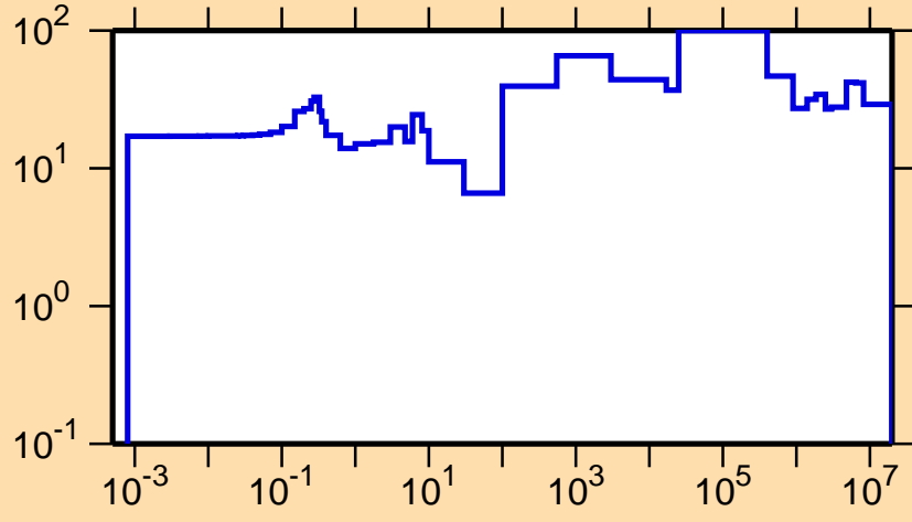
\Delta\sigma/\sigma vs. E for ^{146}\text{Pm}(n,\text{el.})
