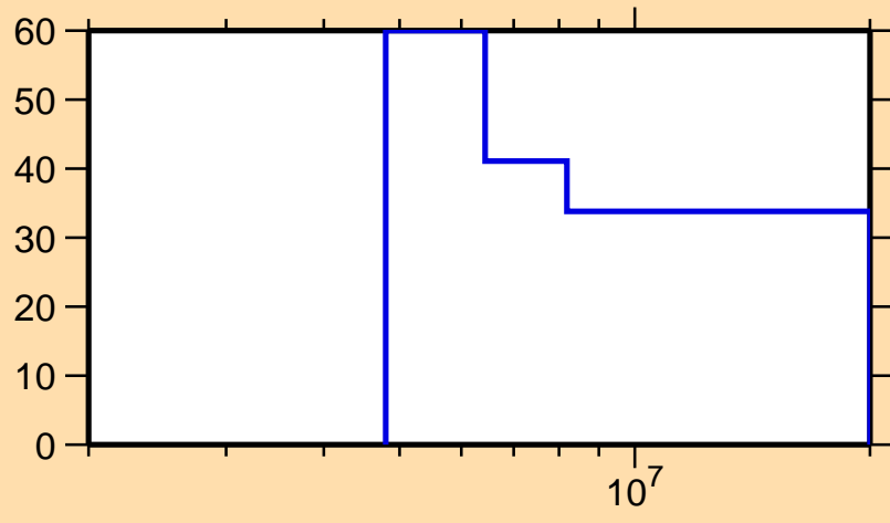
\Delta\sigma/\sigma vs. E for ^{146}\text{Pm}(n,2n)
