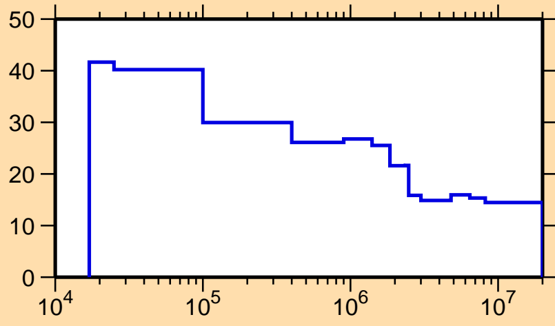
\Delta\sigma/\sigma vs. E for ^{146}\text{Pm}(n,\text{nonel.})
