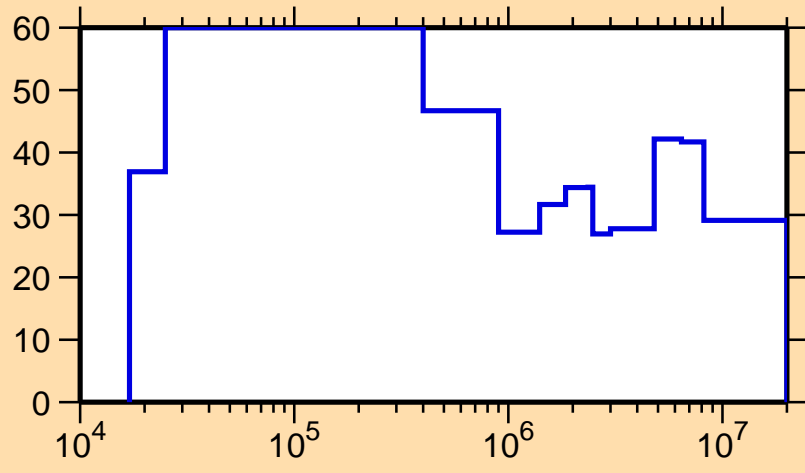
\Delta\sigma/\sigma vs. E for ^{146}\text{Pm}(n,\text{el.})
