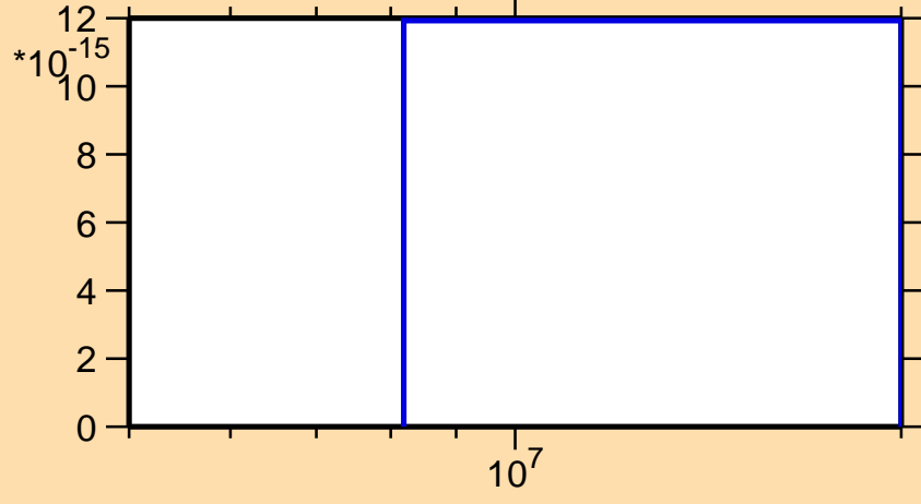
\sigma vs. E for ^{146}\text{Pm} (mt 34)
