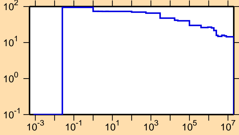
\Delta\sigma/\sigma vs. E for ^{146}\text{Pm}(n,\text{nonel.})
