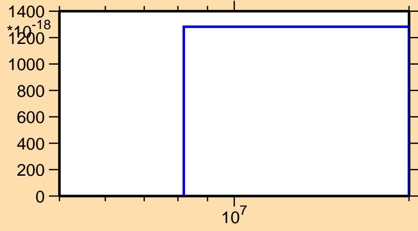
\sigma vs. E for ^{146}\text{Pm} (mt 11)
