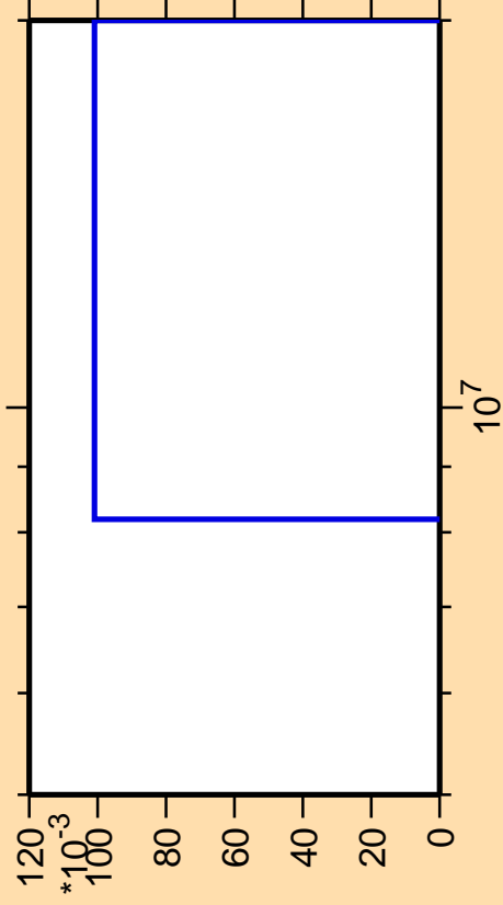
\Delta\sigma/\sigma vs. E for ^{146}\text{Pm} (mt 34)
