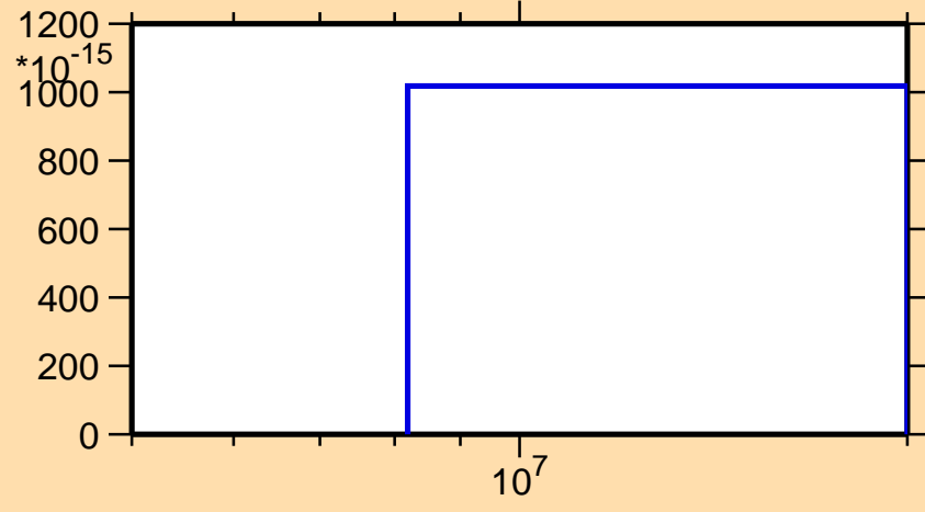
\sigma vs. E for ^{146}\text{Pm} (mt 45)
