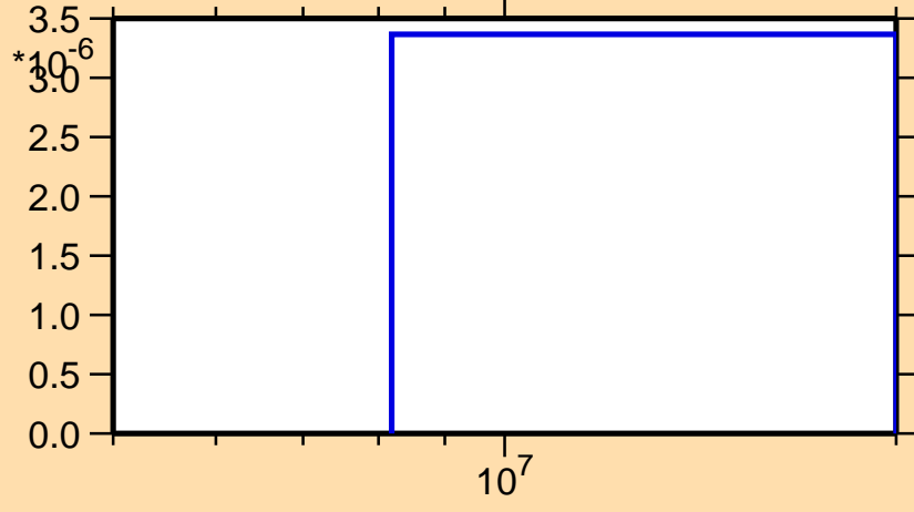
\sigma vs. E for ^{146}\text{Pm}(n,nd)
