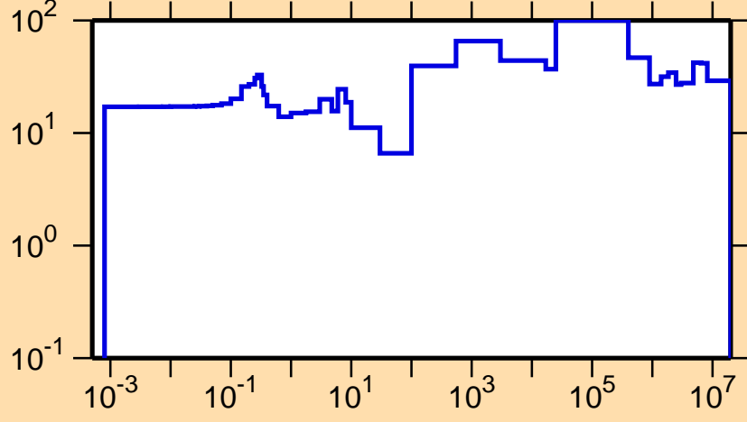
\Delta\sigma/\sigma vs. E for ^{146}\text{Pm}(n,el.)
