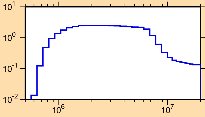
\sigma vs. E for ^{148}\text{Pm}(n,n\text{cont.})
