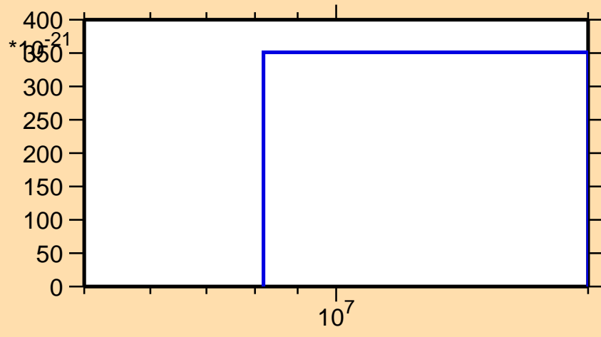
\sigma vs. E for ^{148}\text{Pm} (mt 42)
