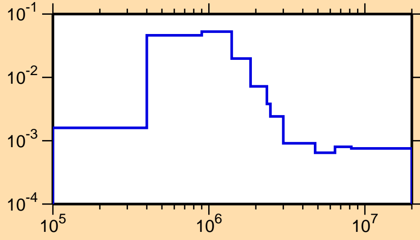
\sigma vs. E for ^{148}\text{Pm}(n,n_3)
