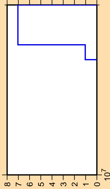
\Delta\sigma/\sigma vs. E for ^{148}\text{Pm}(\text{mt117})
