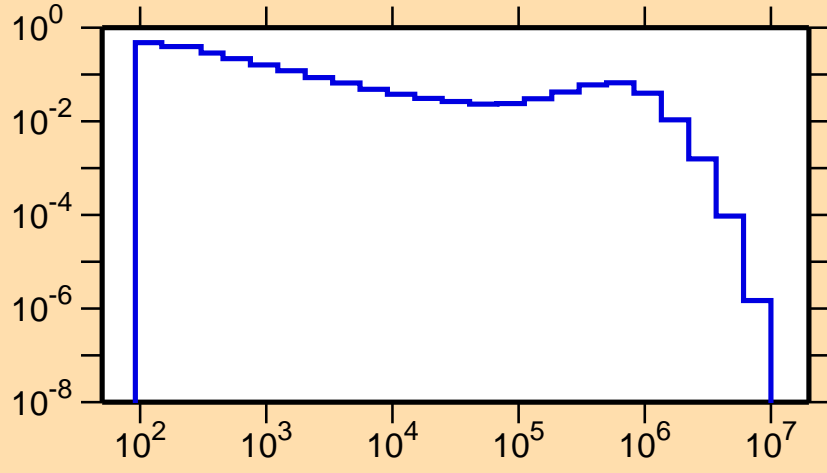
\sigma vs. E for ^{148}\text{Pm}(n,n_2)
