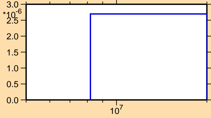
\sigma vs. E for ^{148}\text{Pm}(n,nd)
