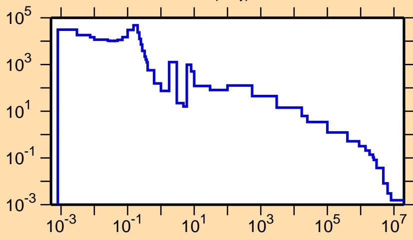
\sigma vs. E for ^{148}\text{Pm}(n,\gamma)
