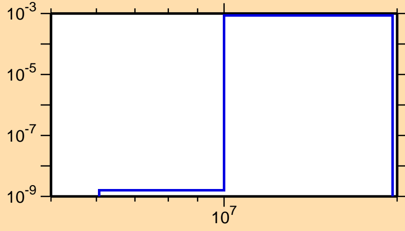
\sigma vs. E for ^{150}\text{Pm}(n,np)
