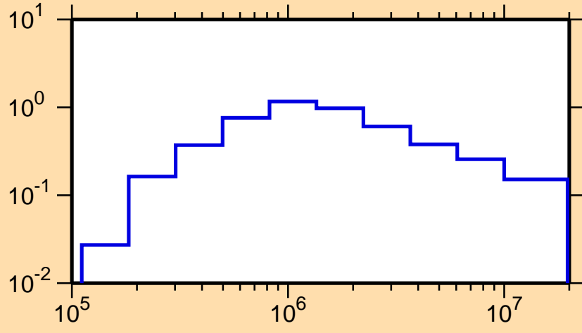
\sigma vs. E for ^{150}\text{Pm}(n,n_3)
