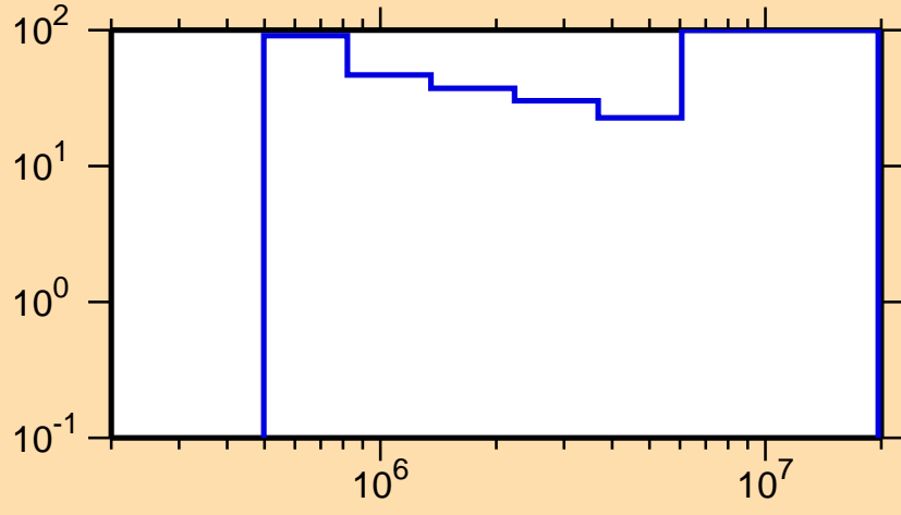
\Delta\sigma/\sigma vs. E for ^{150}\text{Pm}(n,n\text{cont.})
