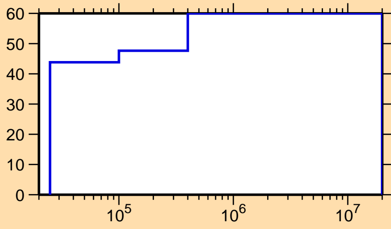
\Delta\sigma/\sigma vs. E for ^{150}\text{Pm}(n,n_1)
