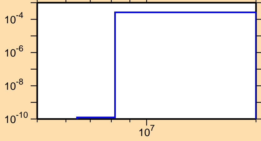
\sigma vs. E for ^{150}\text{Pm}(n,t)
