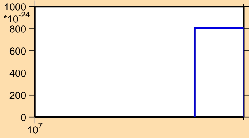
\sigma vs. E for ^{151}\text{Pm} (mt 42)
