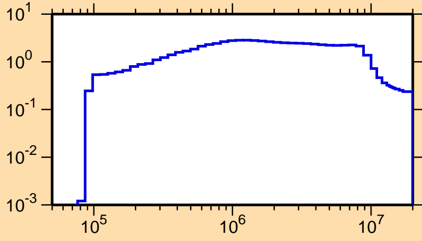
\sigma vs. E for ^{151}\text{Pm}(n,\text{inel.})
