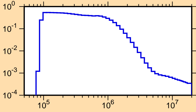
\sigma vs. E for ^{151}\text{Pm}(n,n_1)
