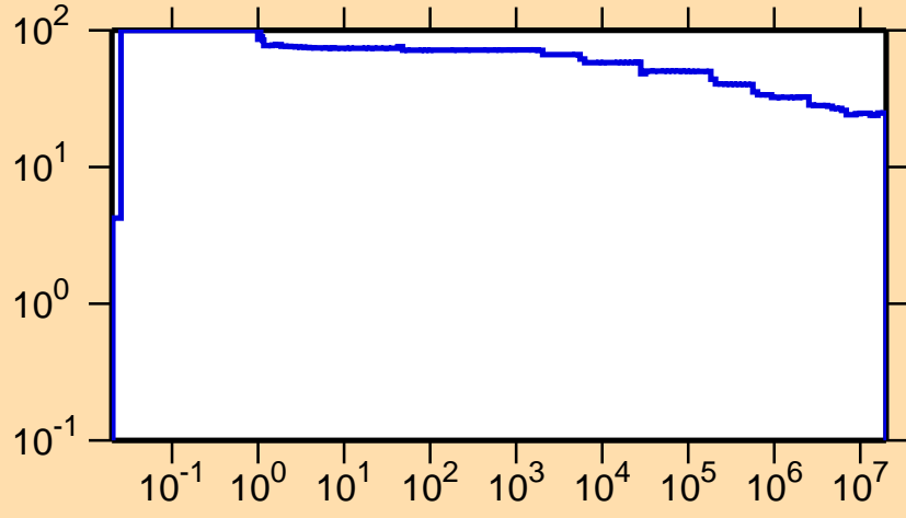
\Delta\sigma/\sigma vs. E for ^{151}\text{Pm}(n,\text{nonel.})
