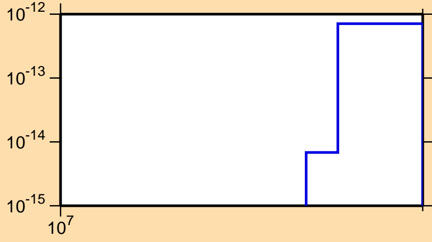
\sigma vs. E for ^{151}\text{Pm}(n,3n\alpha)
