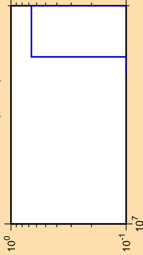
\Delta\sigma/\sigma vs. E for ^{151}\text{Pm}(n,3n\alpha)
