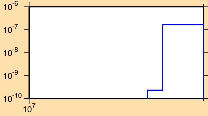
\sigma vs. E for ^{151}\text{Pm}(n,2np)
