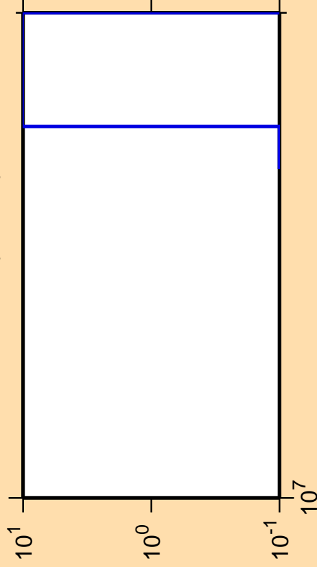
\Delta\sigma/\sigma vs. E for ^{151}\text{Pm}(n,\text{He}3)
