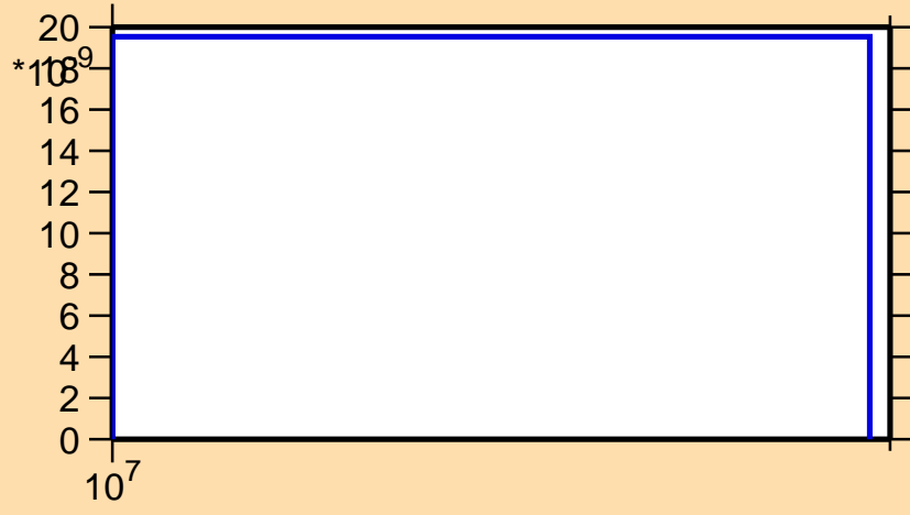
\sigma vs. E for ^{151}\text{Pm}(n,nd)
