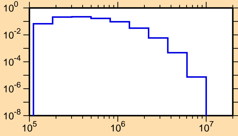
\sigma vs. E for ^{151}\text{Pm}(n,n_2)
