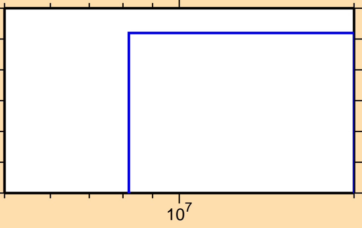
\sigma vs. E for ^{151}\text{Pm}(n,nt)
