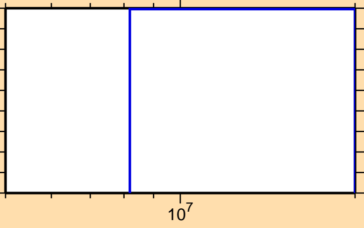
\sigma vs. E for ^{151}\text{Pm}(n,nd)
