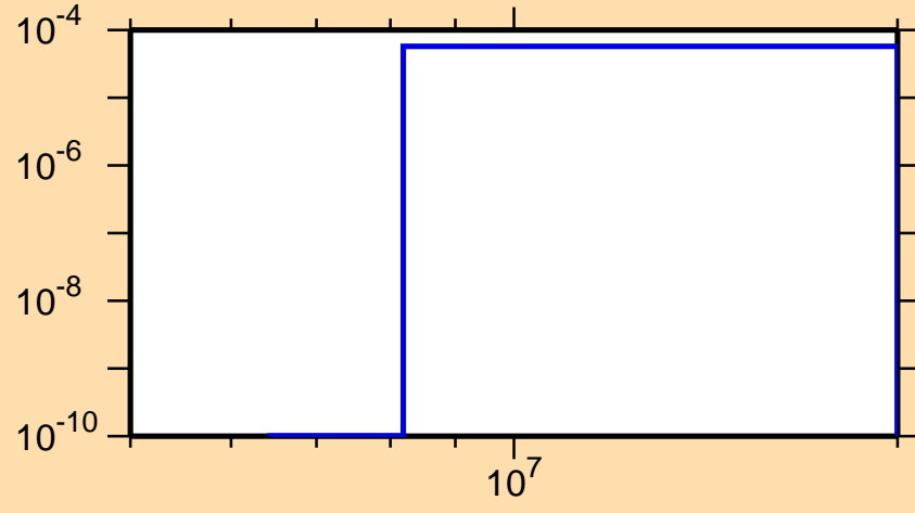
\sigma vs. E for ^{151}\text{Pm}(n,n\alpha)
