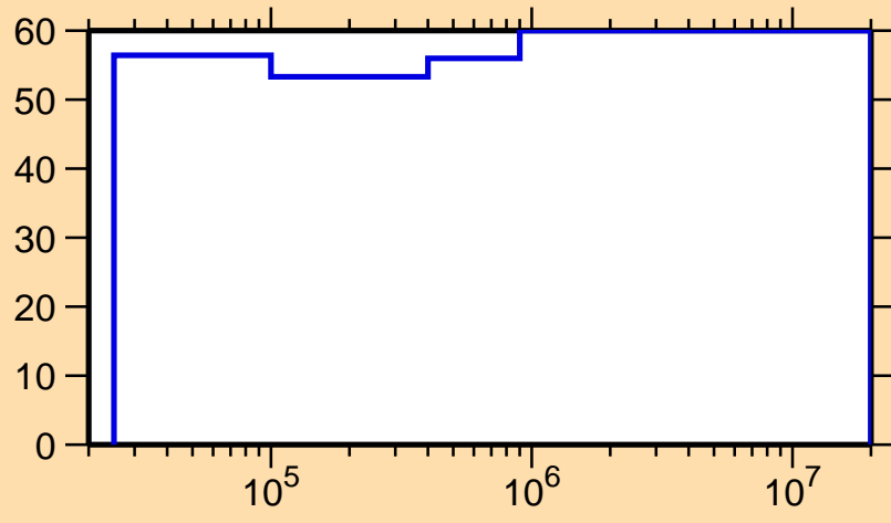
\Delta\sigma/\sigma vs. E for ^{151}\text{Pm}(n,n_1)
