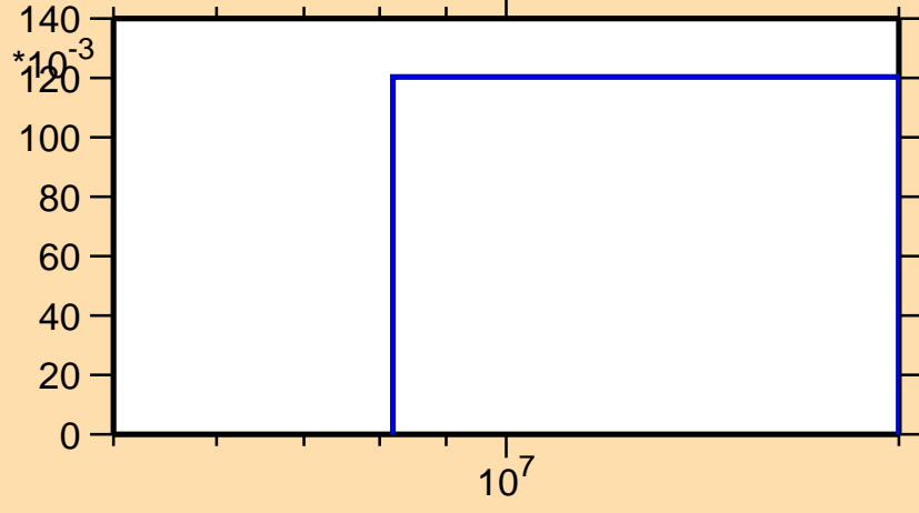
\sigma vs. E for ^{151}\text{Pm}(n,3n)
