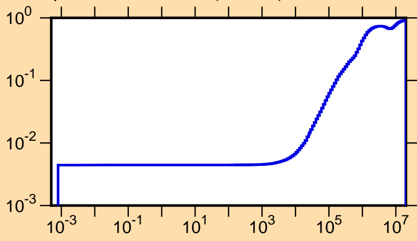
\mu vs. E for ^{152}\text{Pm}(\text{mt251})
