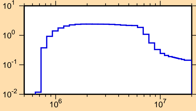
\sigma vs. E for ^{152}\text{Pm}(n,n\text{cont.})
