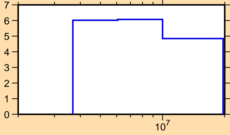
\Delta\sigma/\sigma vs. E for ^{152}\text{Pm}(n,\text{nonel.})
