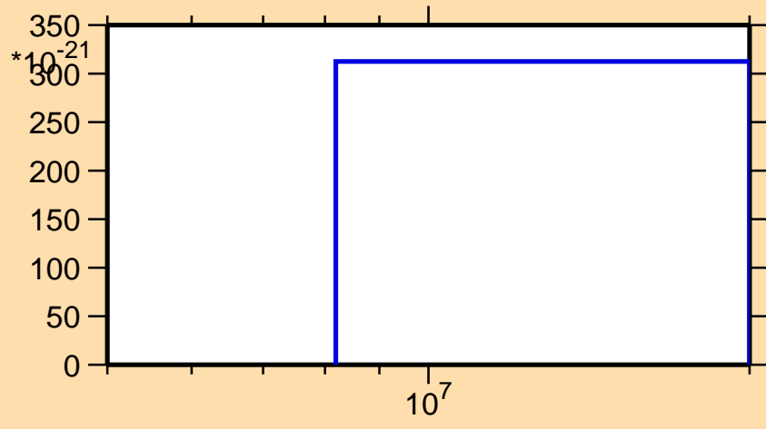
\sigma vs. E for ^{152}\text{Pm} (mt 11)
