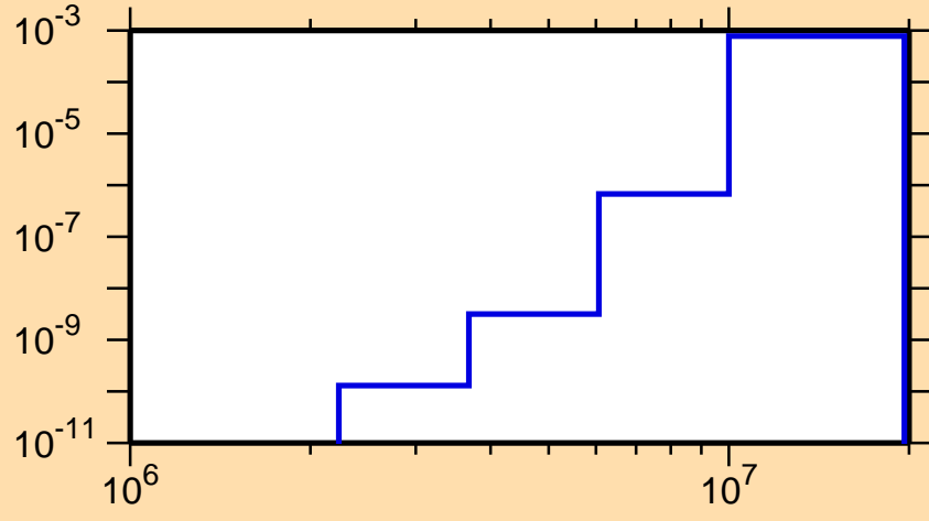
\sigma vs. E for ^{152}\text{Pm}(n,\alpha)
