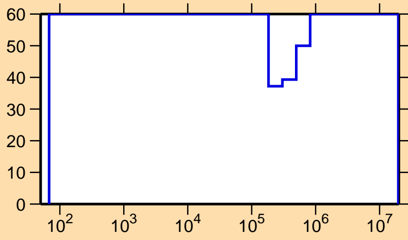
\Delta\sigma/\sigma vs. E for ^{152}\text{Pm}(n,n_1)
