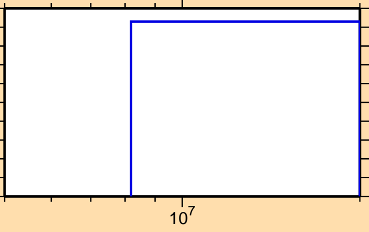
\sigma vs. E for ^{154}\text{Pm} (mt 11)
