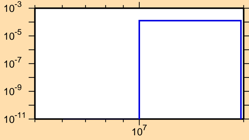
\sigma vs. E for ^{155}\text{Pm}(n,d)
