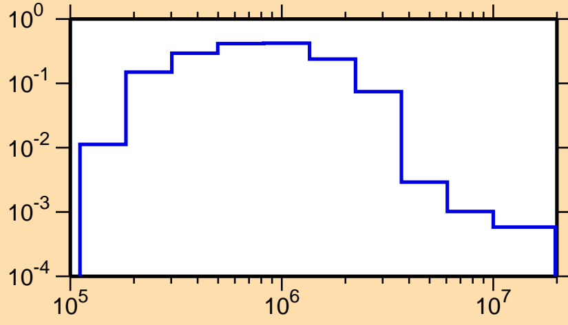
\sigma vs. E for ^{155}\text{Pm}(n,n_2)
