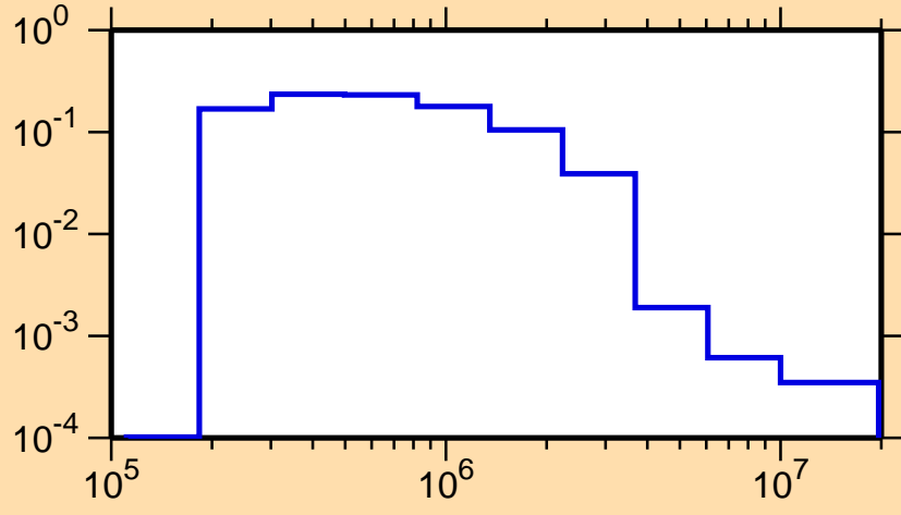
\sigma vs. E for ^{155}\text{Pm}(n,n_3)
