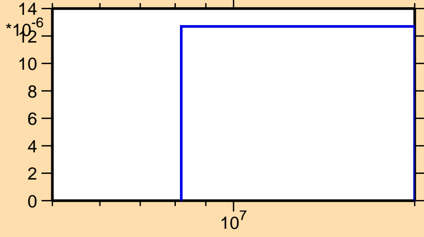
\sigma vs. E for ^{155}\text{Pm}(n,t)
