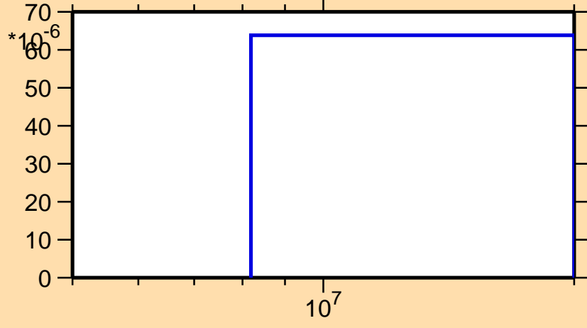
\sigma vs. E for ^{155}\text{Pm}(n,np)
