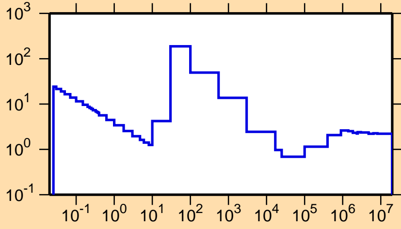
\sigma vs. E for ^{155}\text{Pm}(n,\text{nonel.})
