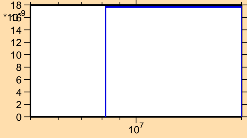
\sigma vs. E for ^{155}\text{Pm}(n,nt)
