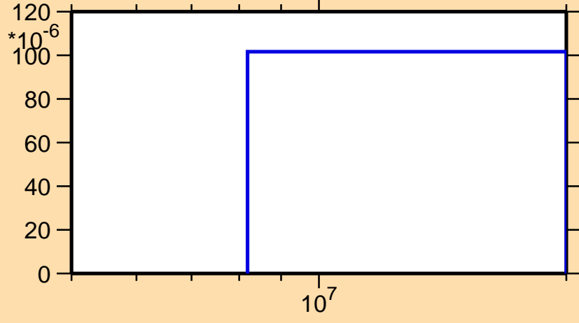
\sigma vs. E for ^{155}\text{Pm}(n,d)
