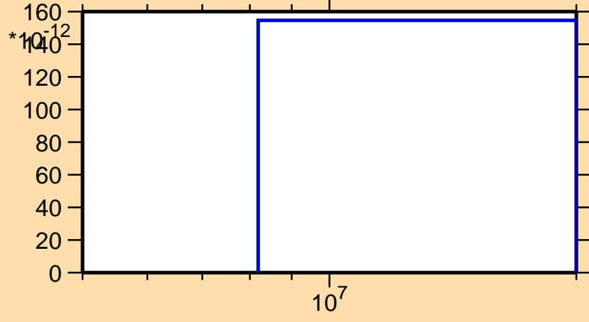
\sigma vs. E for ^{155}\text{Pm}(n,2np)
