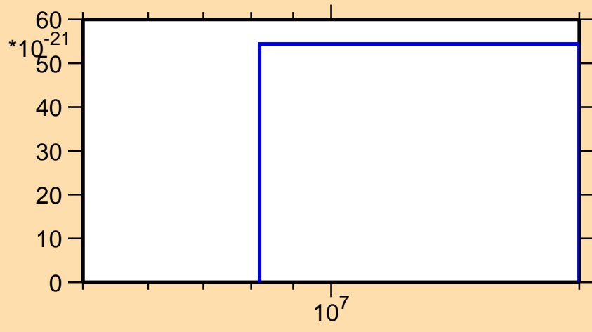
\sigma vs. E for ^{155}\text{Pm} (mt 11)
