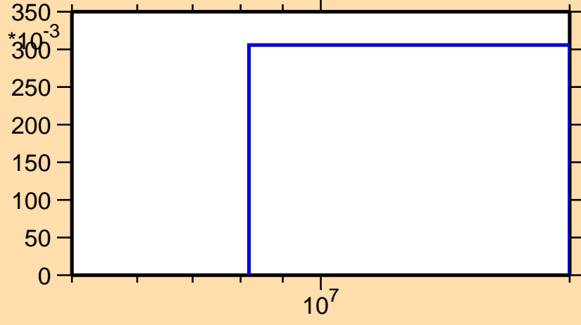
\sigma vs. E for ^{155}\text{Pm}(n,3n)
