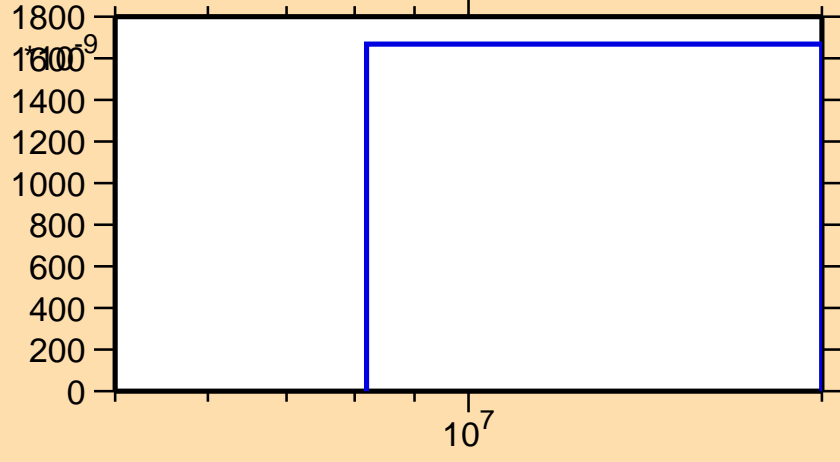
\sigma vs. E for ^{155}\text{Pm}(n,n\alpha)
