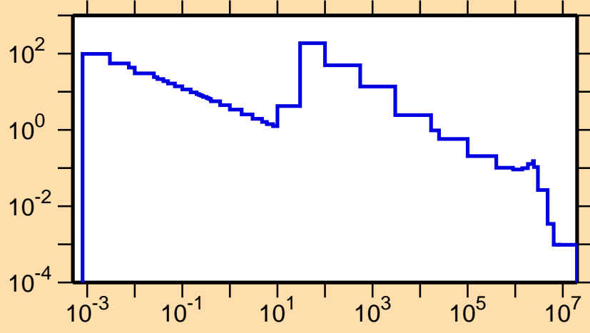
\sigma vs. E for ^{155}\text{Pm}(n,\gamma)
