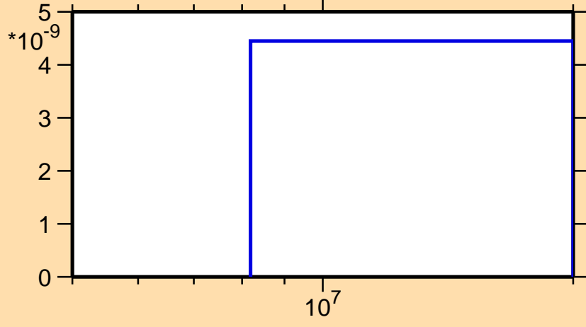
\sigma vs. E for ^{155}\text{Pm}(n,nd)
