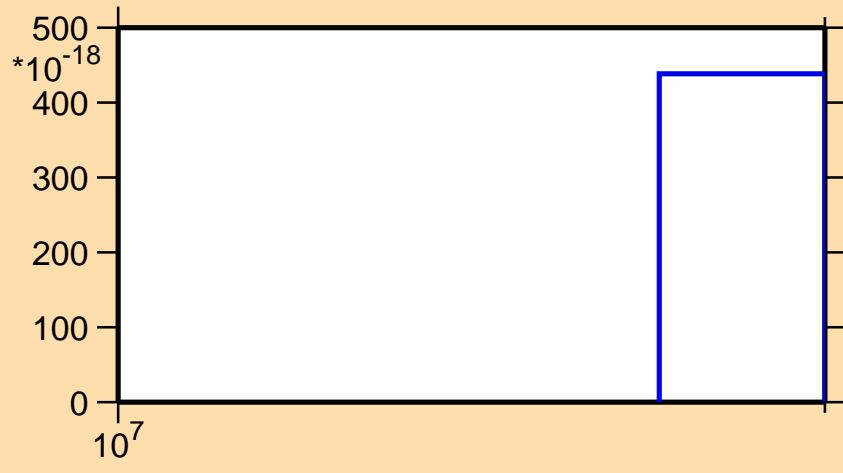
\sigma vs. E for ^{156}\text{Pm} (mt 11)
