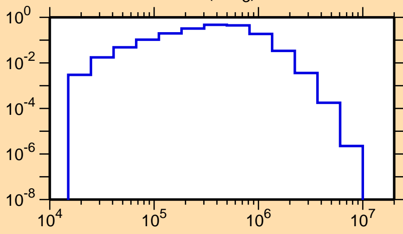
\sigma vs. E for ^{156}\text{Pm}(n,n_3)
