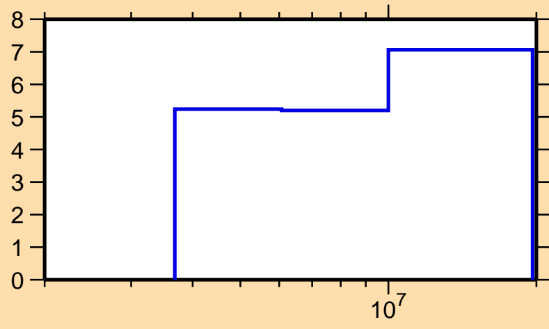
\Delta\sigma/\sigma vs. E for ^{156}\text{Pm}(n,\text{nonel.})
