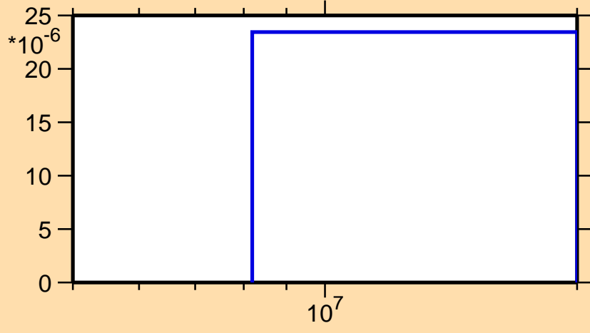
\sigma vs. E for ^{156}\text{Pm}(n,t)
