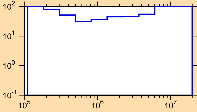
\Delta\sigma/\sigma vs. E for ^{158}\text{Pm}(n,n\text{cont.})
