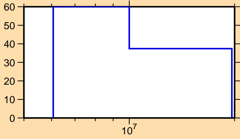
\Delta\sigma/\sigma vs. E for ^{158}\text{Pm}(n,el.)
