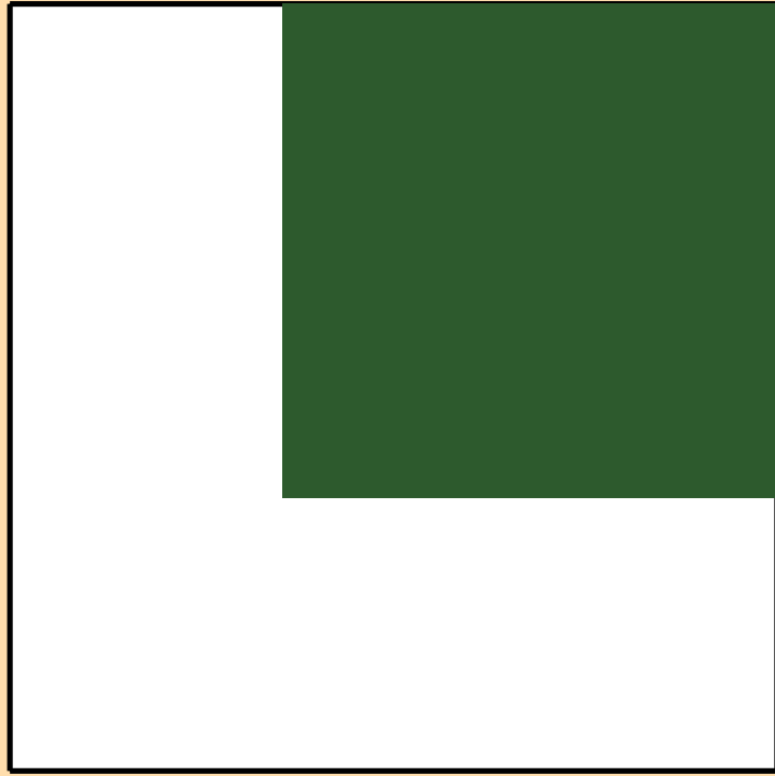
\sigma vs. E for ^{158}\text{Pm}(n,t)
