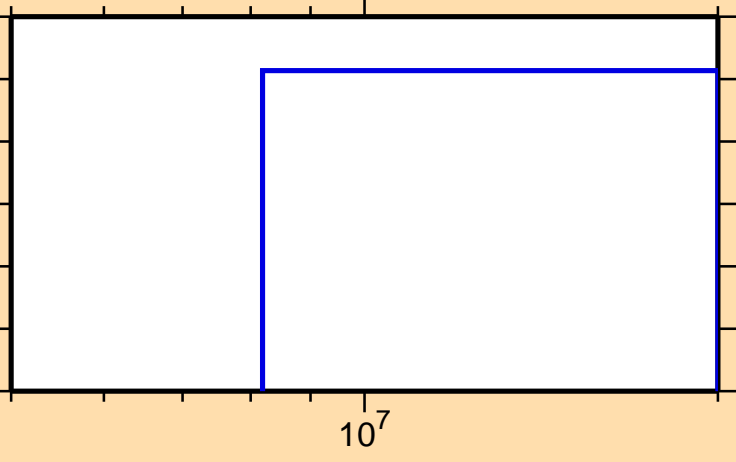
\sigma vs. E for ^{158}\text{Pm}(n,np)
