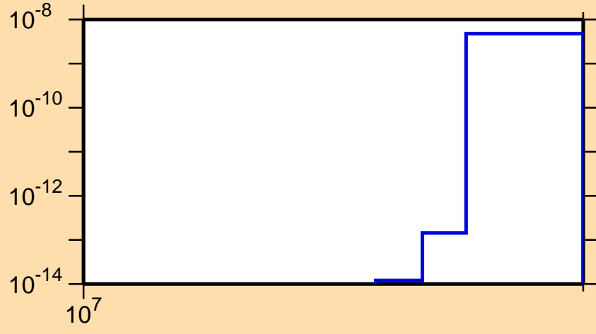
\sigma vs. E for ^{159}\text{Pm}(n,2np)
