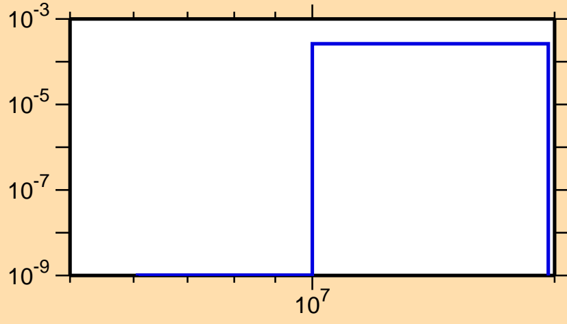
\sigma vs. E for ^{159}\text{Pm}(n,p)
