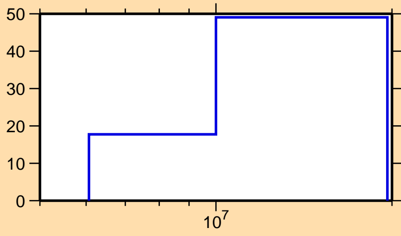
\Delta\sigma/\sigma vs. E for ^{159}\text{Pm}(n,2n)
