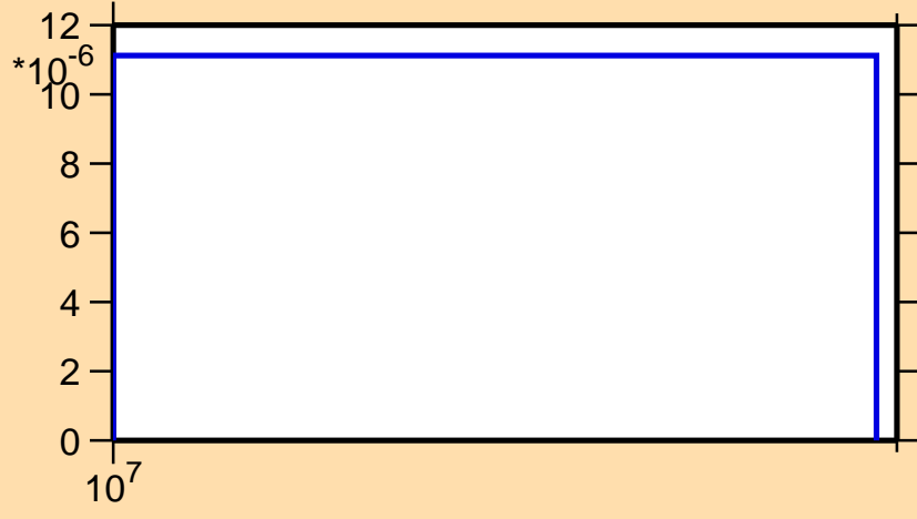
\sigma vs. E for ^{159}\text{Pm}(n,np)
