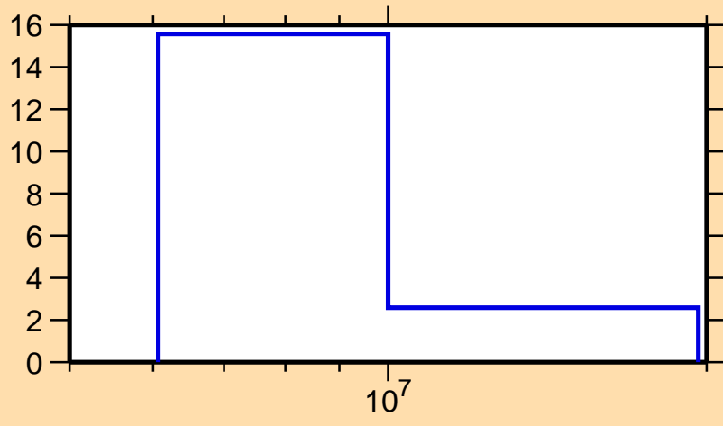
\Delta\sigma/\sigma vs. E for ^{159}\text{Pm}(n,\text{tot.})
