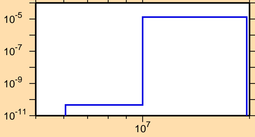
\sigma vs. E for ^{159}\text{Pm}(n,\alpha)
