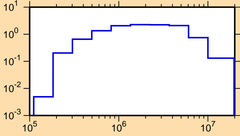
\sigma vs. E for ^{159}\text{Pm}(n,n\text{cont.})
