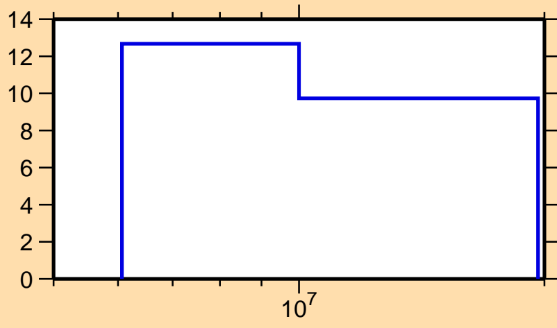
\Delta\sigma/\sigma vs. E for ^{159}\text{Pm}(n,\text{nonel.})
