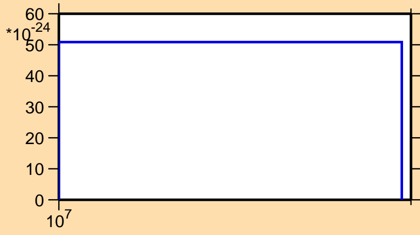
\sigma vs. E for ^{159}\text{Pm} (mt 42)
