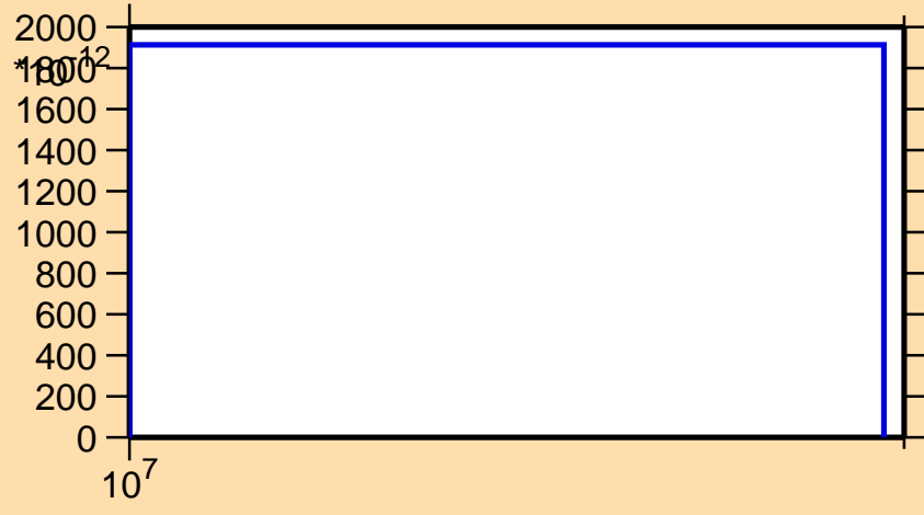
\sigma vs. E for ^{159}\text{Pm}(n,\text{nd})
