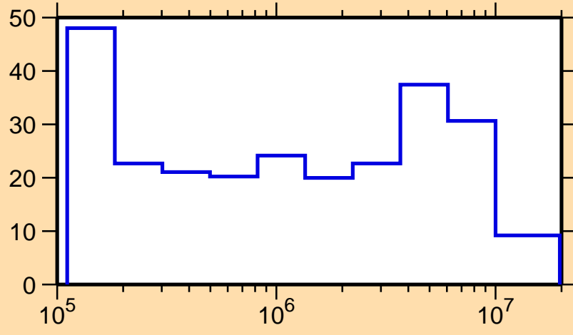
\Delta\sigma/\sigma vs. E for ^{159}\text{Pm}(n,\text{el.})
