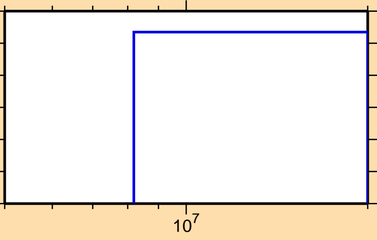
\sigma vs. E for ^{159}\text{Pm} (mt 42)
