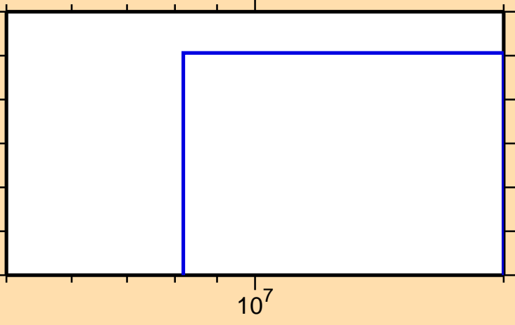
\sigma vs. E for ^{195}\text{Po}(n,nt)
