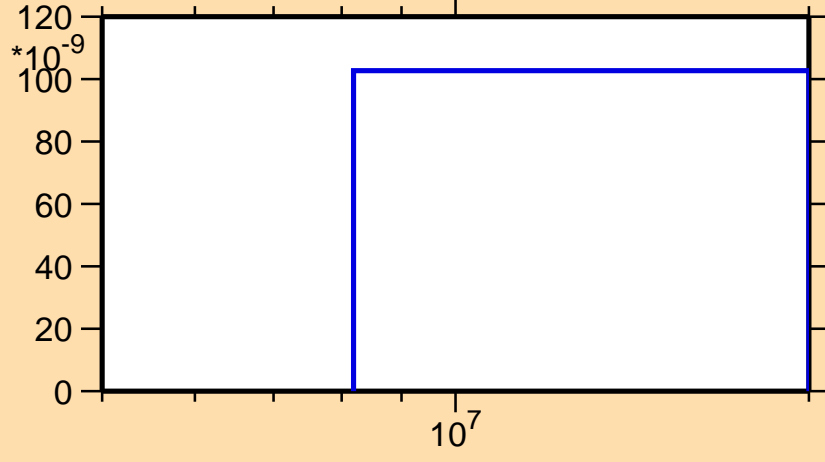
\sigma vs. E for ^{195}\text{Po}(n,\text{pd})
