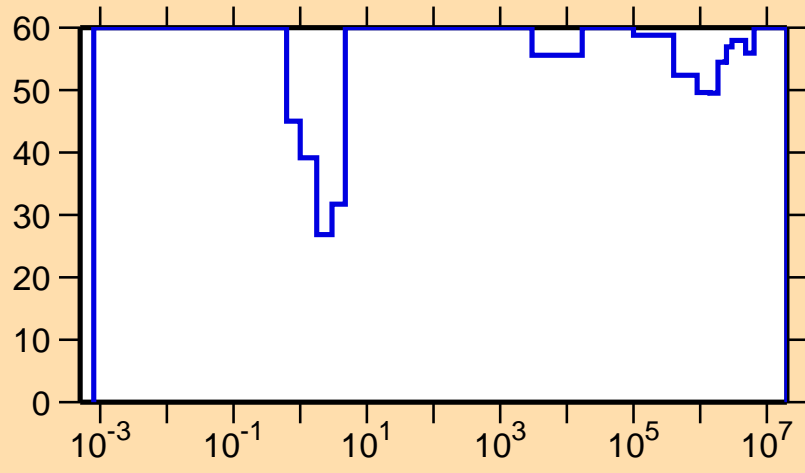
\Delta\sigma/\sigma vs. E for ^{195}\text{Po}(n,\gamma)
