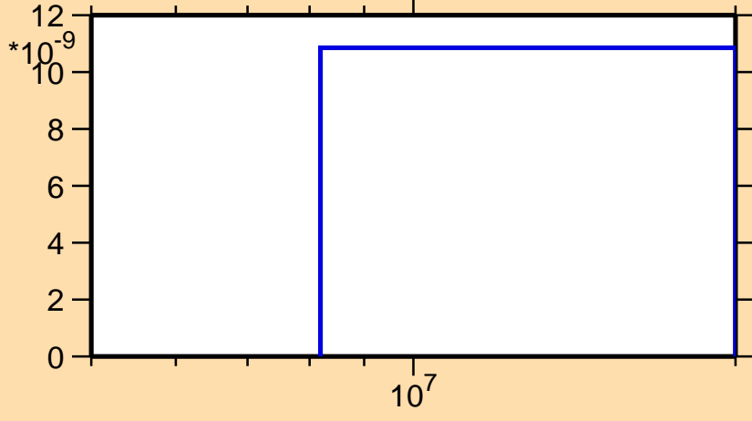
\sigma vs. E for ^{195}\text{Po}(n,\text{pt})
