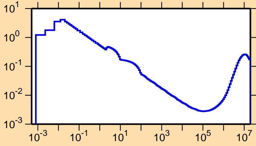
\sigma vs. E for ^{195}\text{Po}(n,p)
