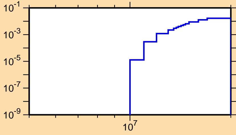
\sigma vs. E for ^{195}\text{Po}(n,2n\alpha)
