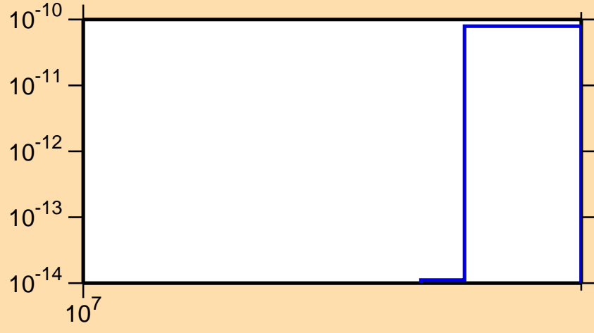
\sigma vs. E for ^{197}\text{Po}(n,nt)
