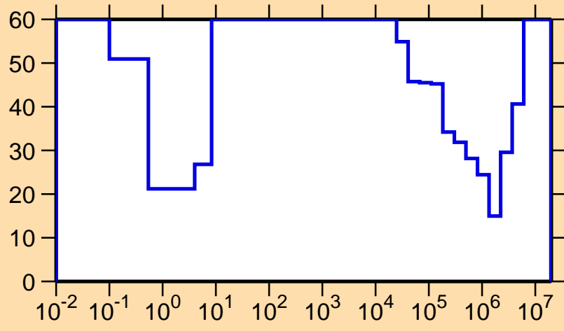
\Delta\sigma/\sigma vs. E for ^{197}\text{Po}(n,\gamma)
