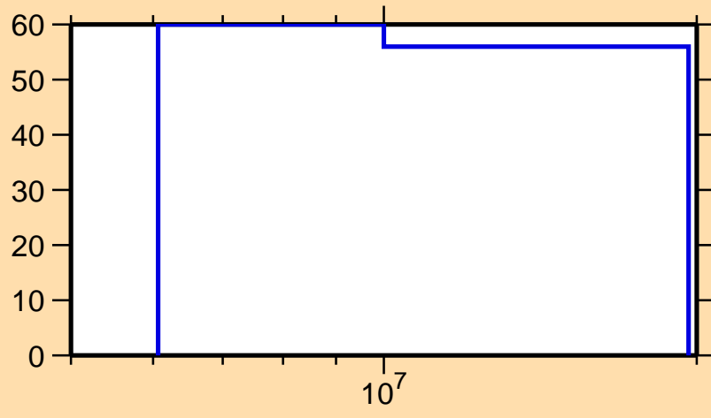
\Delta\sigma/\sigma vs. E for ^{197}\text{Po}(n,2n)
