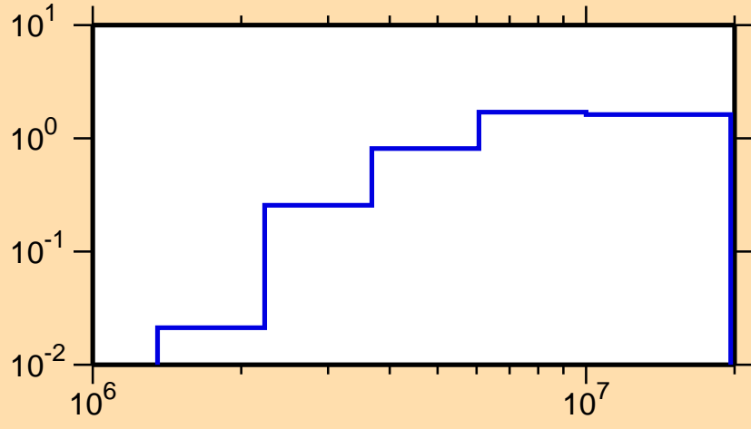
\sigma vs. E for ^{197}\text{Po}(n,n\text{cont.})
