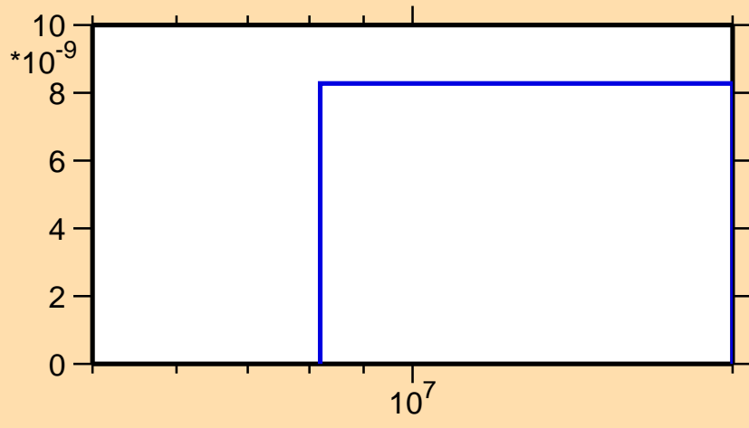
\sigma vs. E for ^{197}\text{Po}(n,\text{pd})
