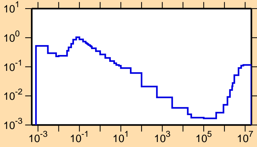
\sigma vs. E for ^{197}\text{Po}(n,p)
