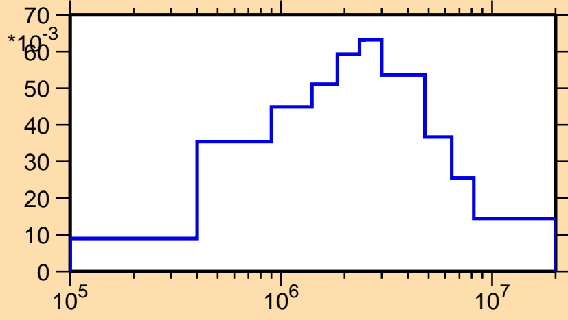
\sigma vs. E for ^{197}\text{Po}(n,n_1)
