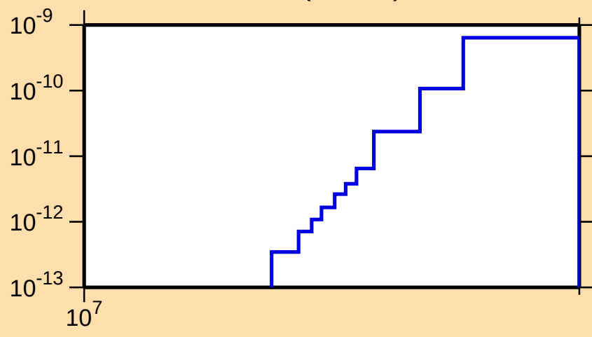
\sigma vs. E for ^{197}\text{Po}(\text{mt117})
