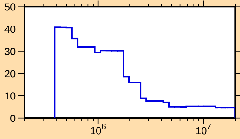
\Delta\sigma/\sigma vs. E for ^{197}\text{Po}(n,n\text{onel.})
