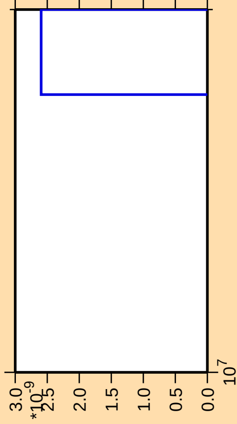
\Delta\sigma/\sigma vs. E for ^{197}\text{Po}(\text{mt } 11)
